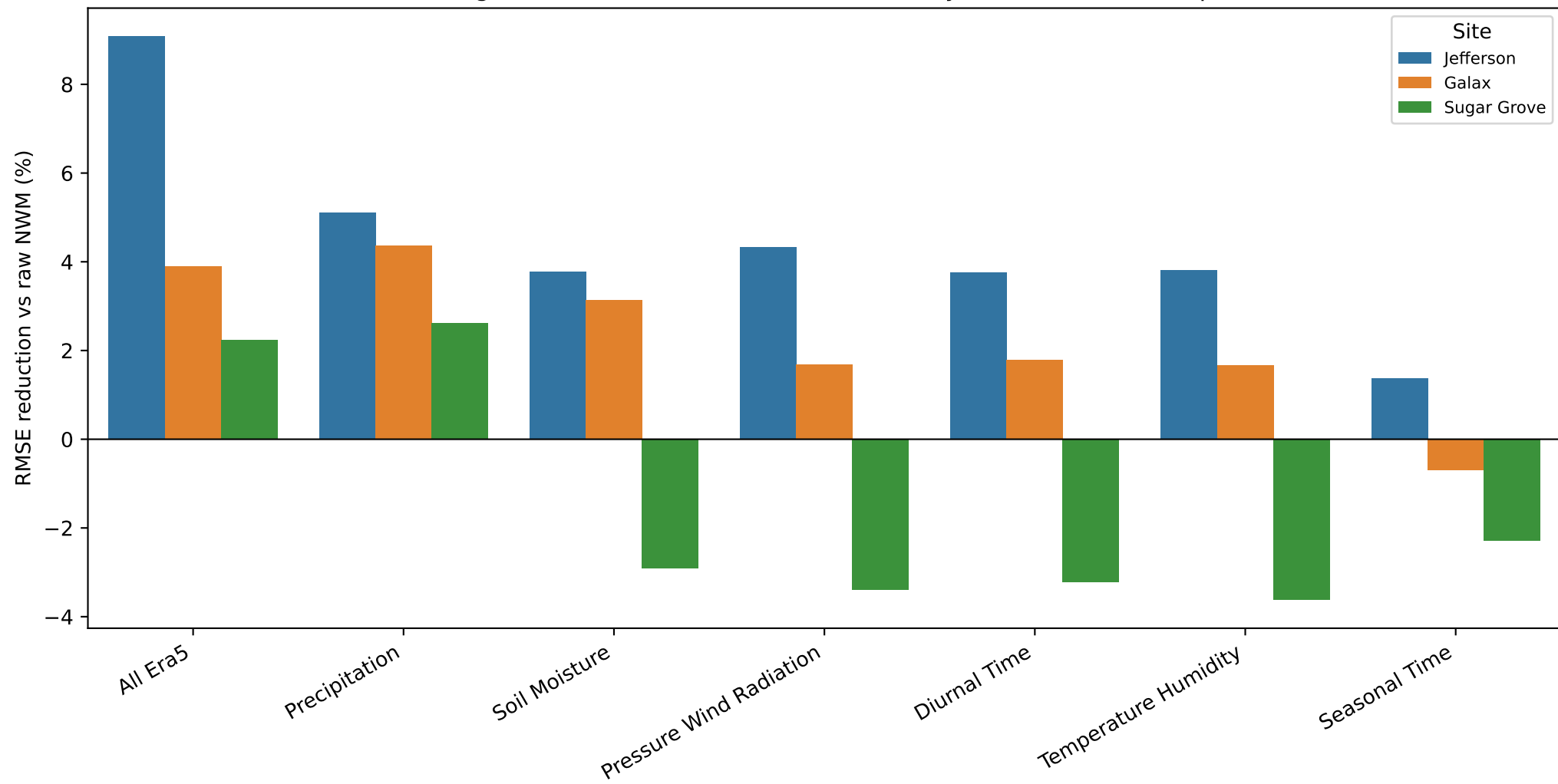
Diagnostic Residual-Model Performance by ERA5 Feature Group
