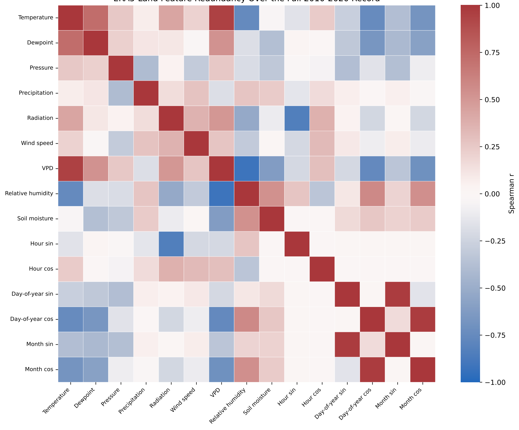
ERA5-Land Feature Redundancy Over the Full 2010-2020 Record
