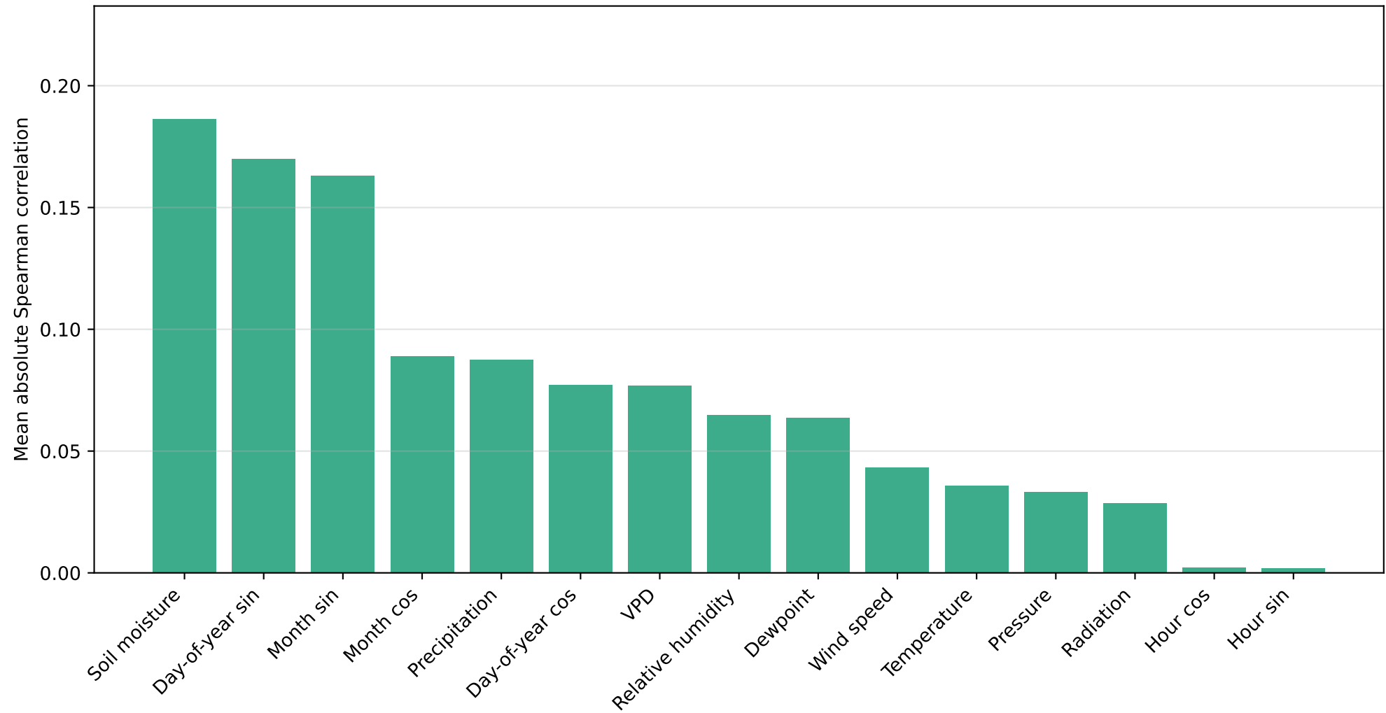
Feature Association With NWM Bias and Absolute Error
