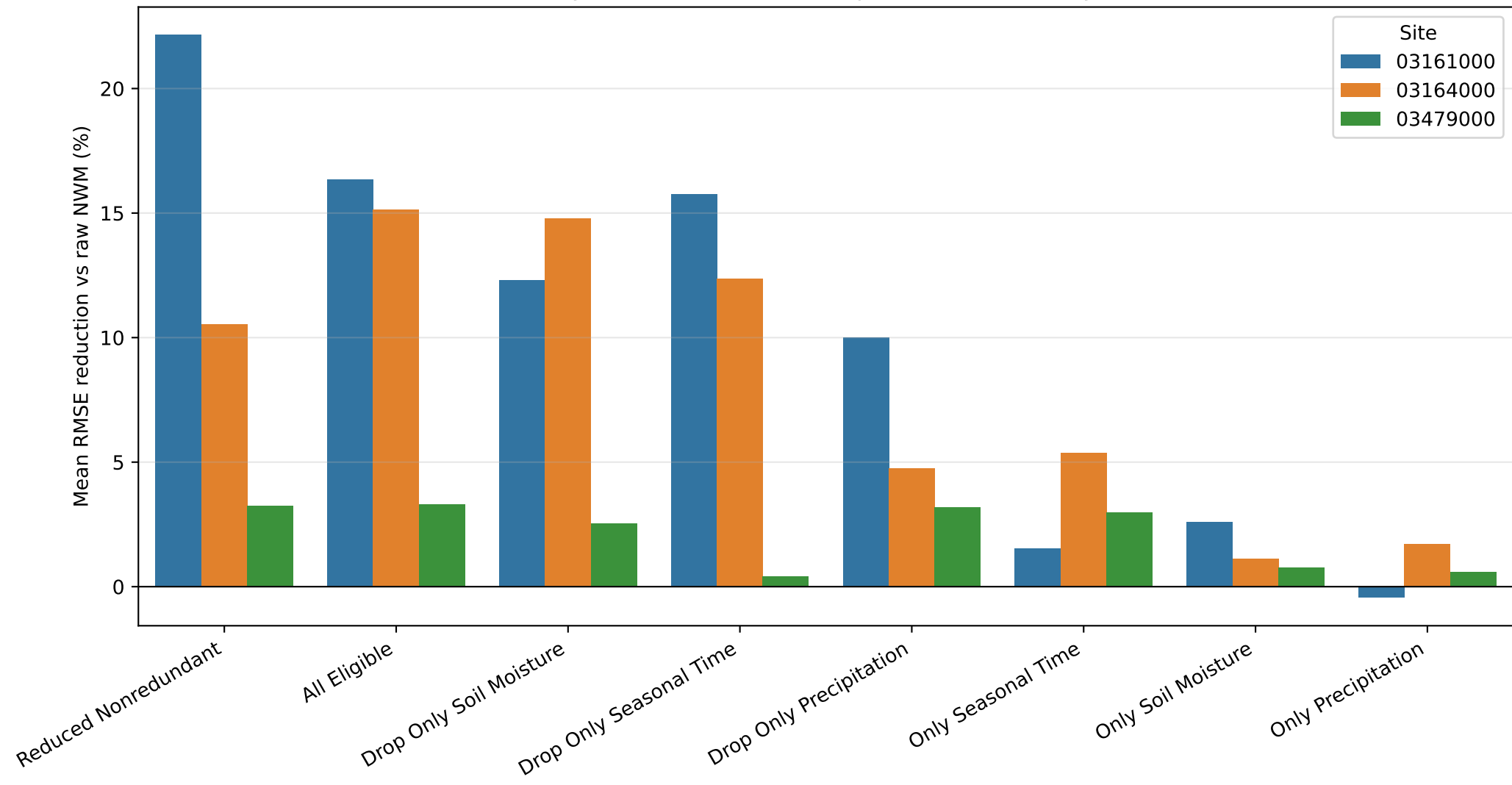
Hydra ERA5 Feature-Group Ablation Summary
