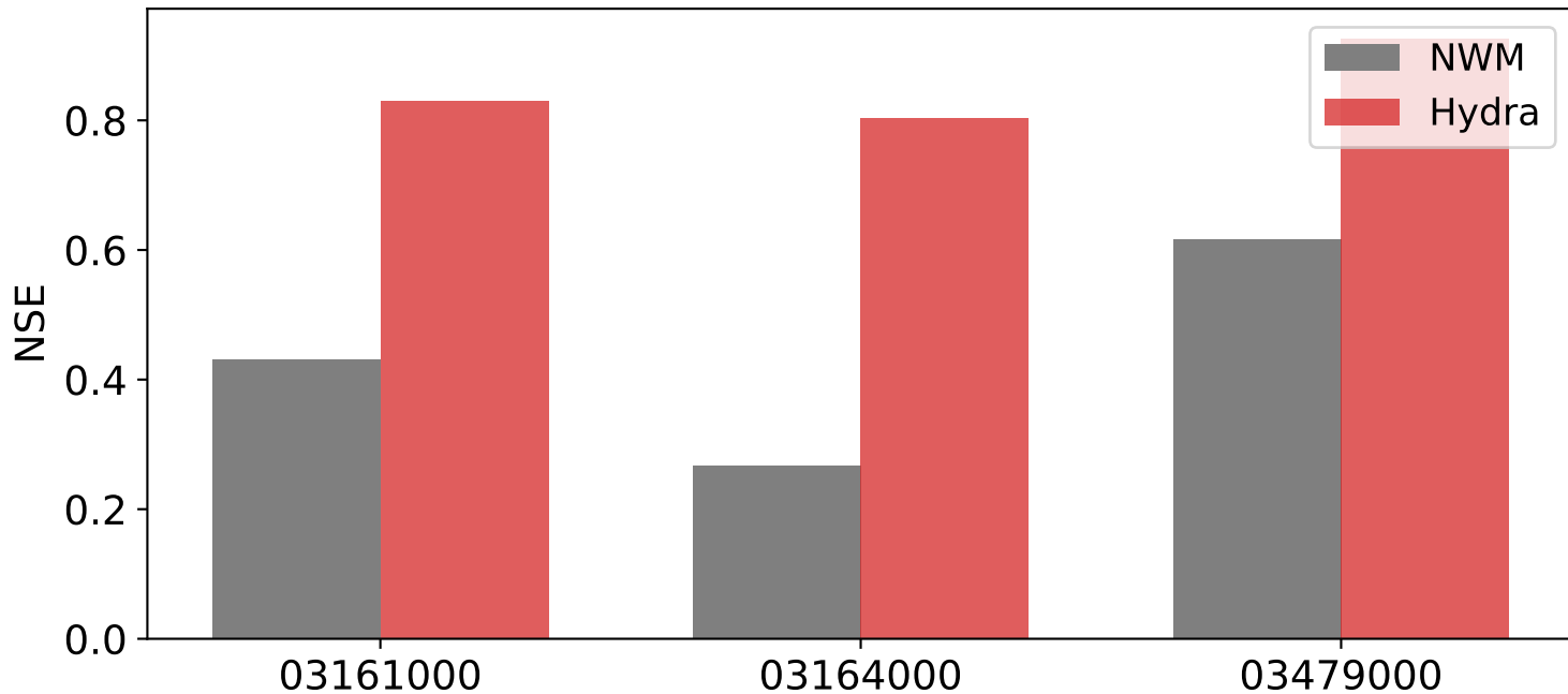
Baseline vs Hydra: NSE
