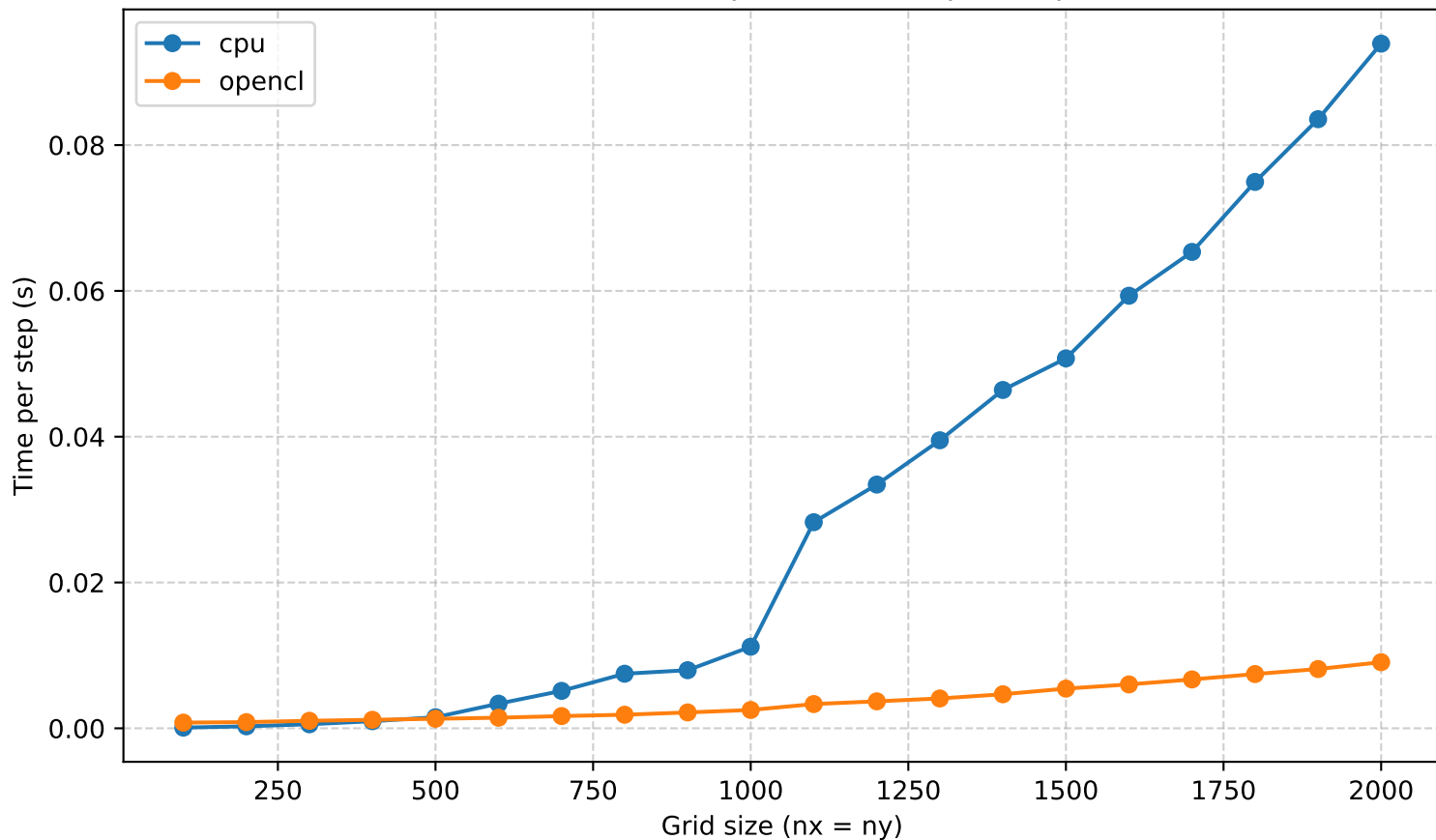
Benchmark comparison (time per step)
