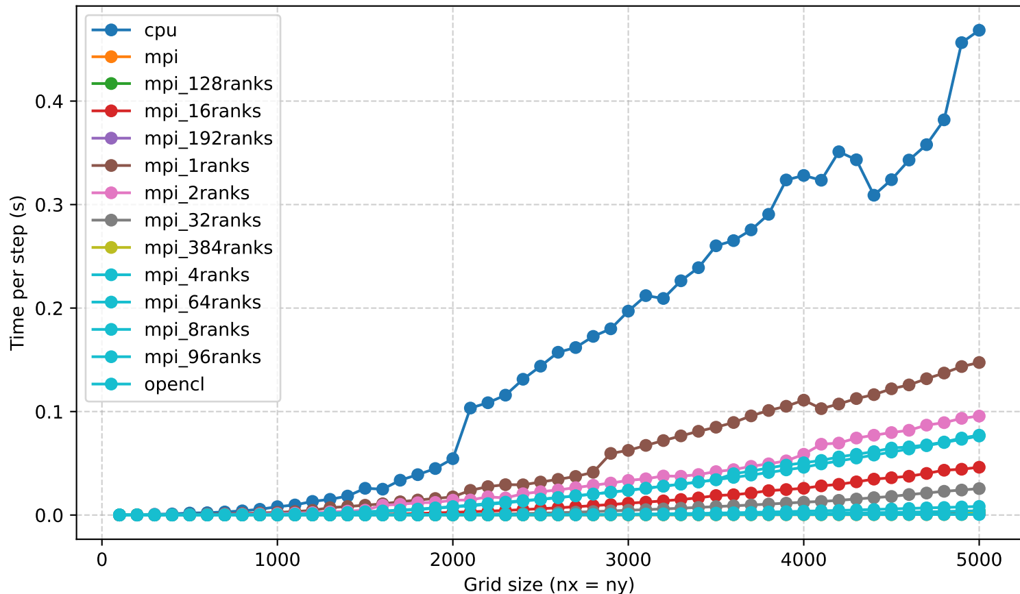
Benchmark comparison (time per step)
