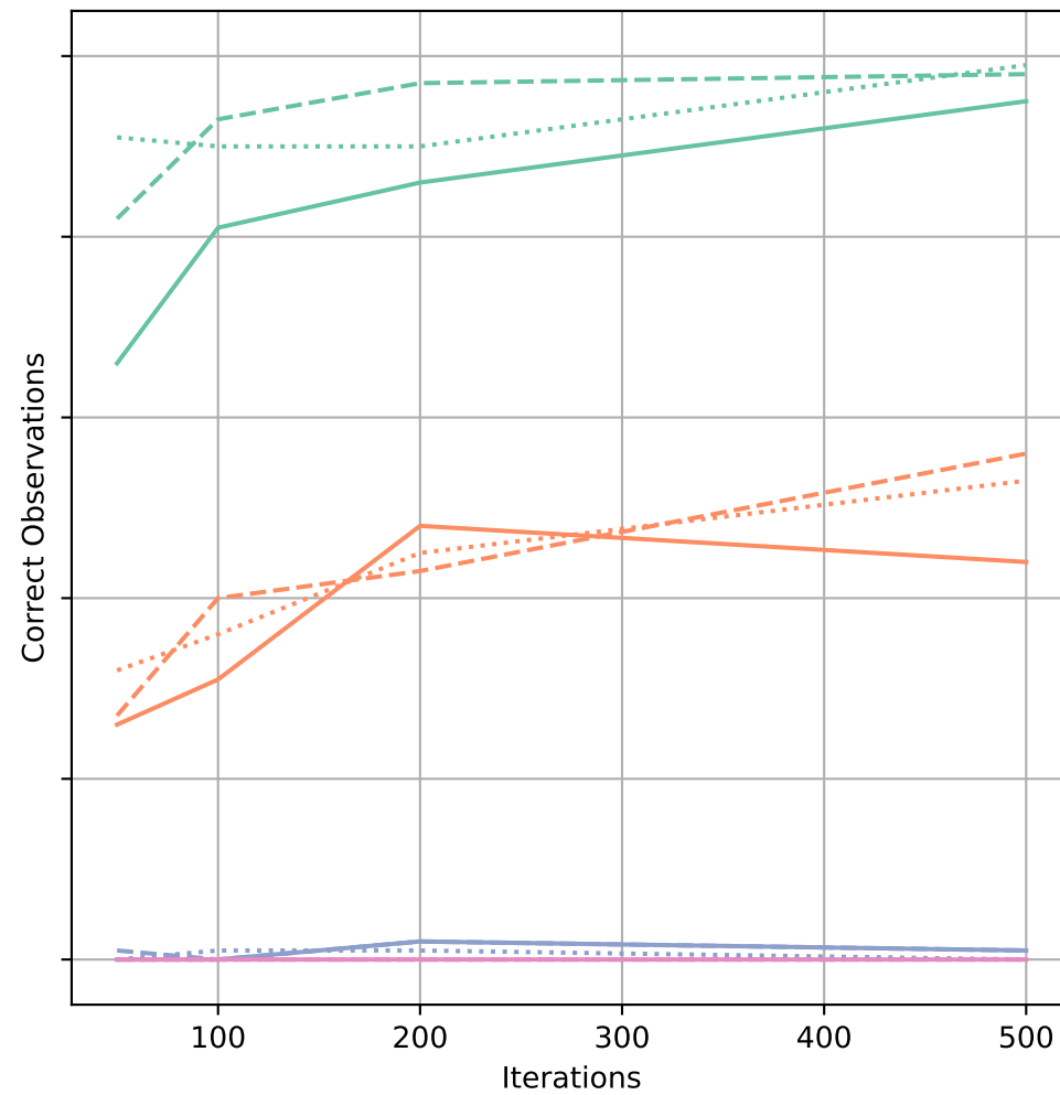
Inlier Deviation: 0.005
