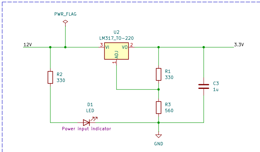
3.3V Circuit
