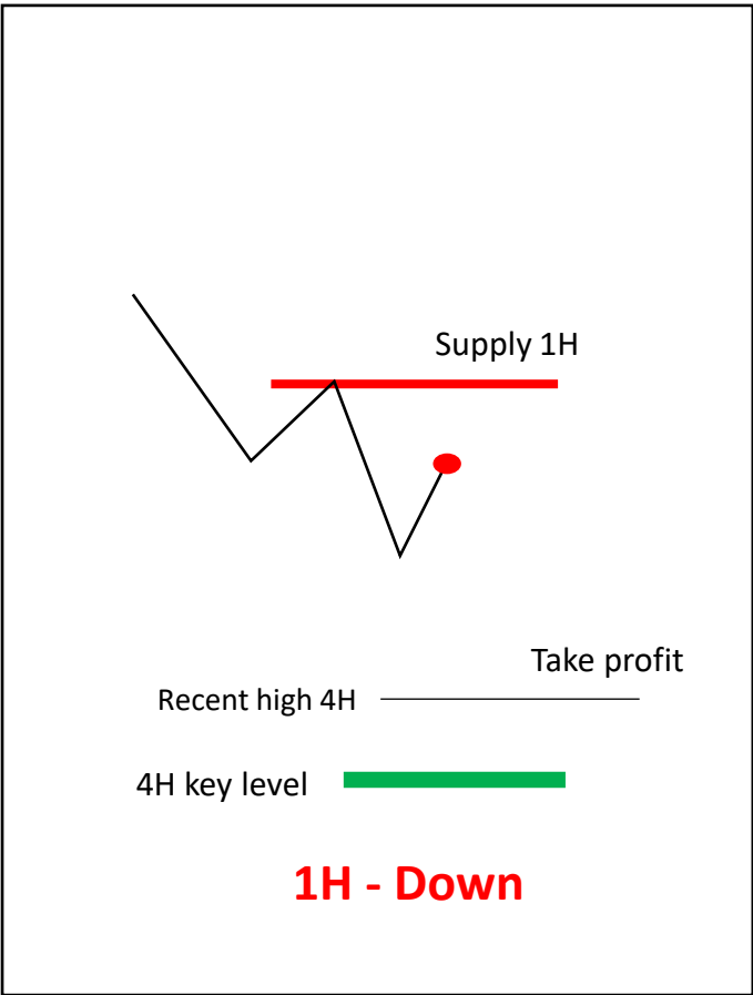
Case 2. All TFs are non-confluence
