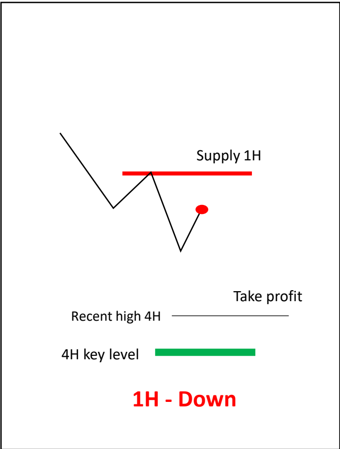
Case 1. At least 2 TFs are confluence
