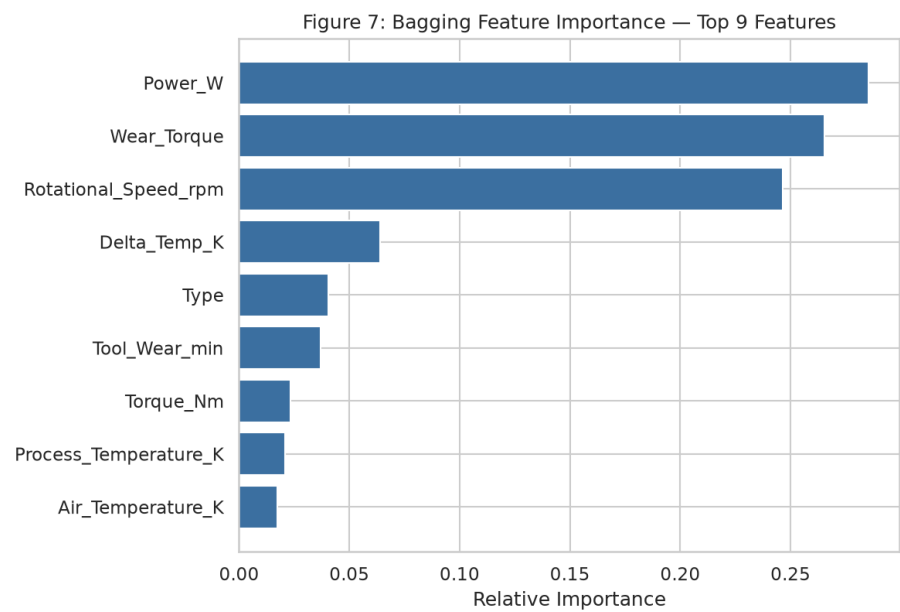
Figure 7: Bagging Feature Importance — Top Features (Mean Across Base Estimators)
