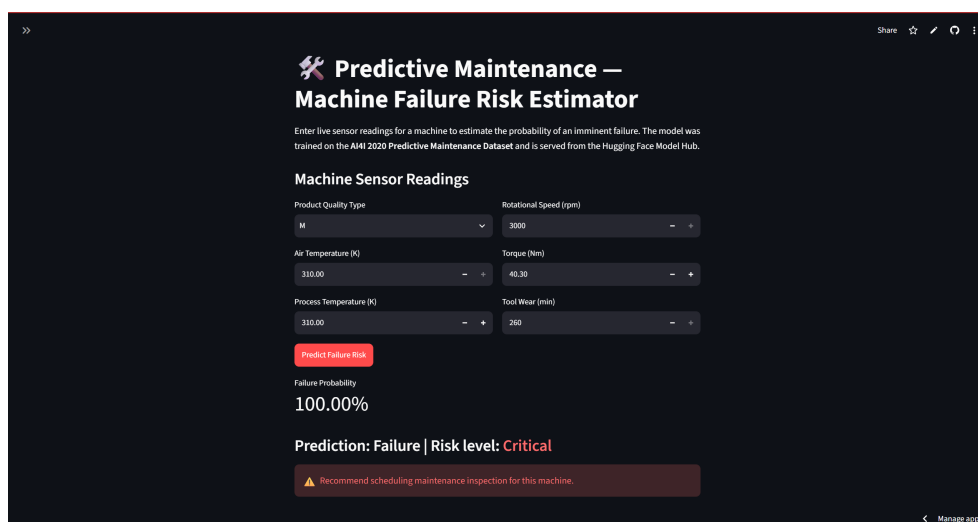
Figure 10: Live Streamlit App — Critical-Risk Prediction (Extreme Sensor Values)
