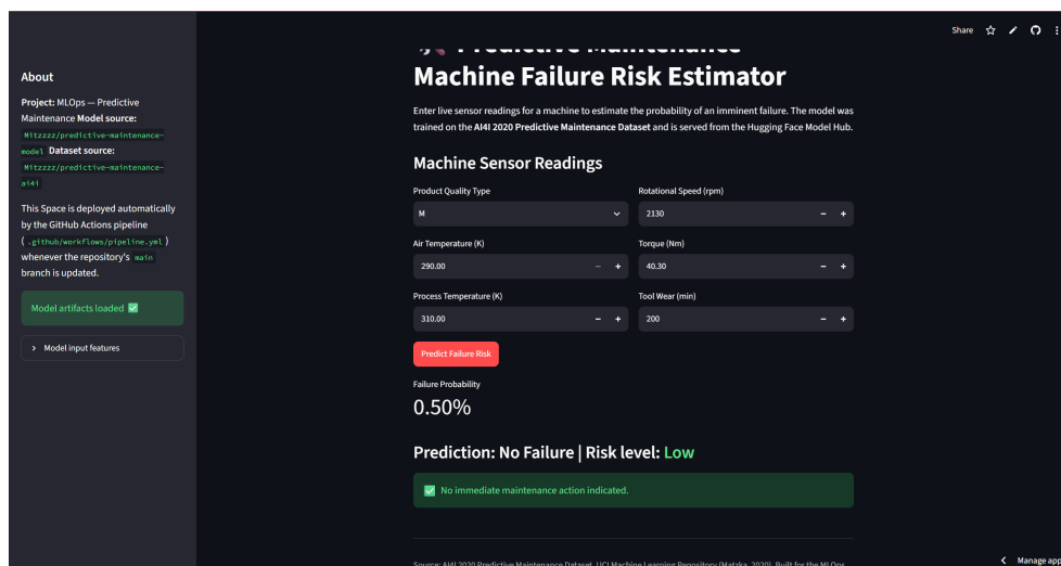
Figure 9: Live Streamlit App — Low-Risk Prediction (Default Sensor Values)
