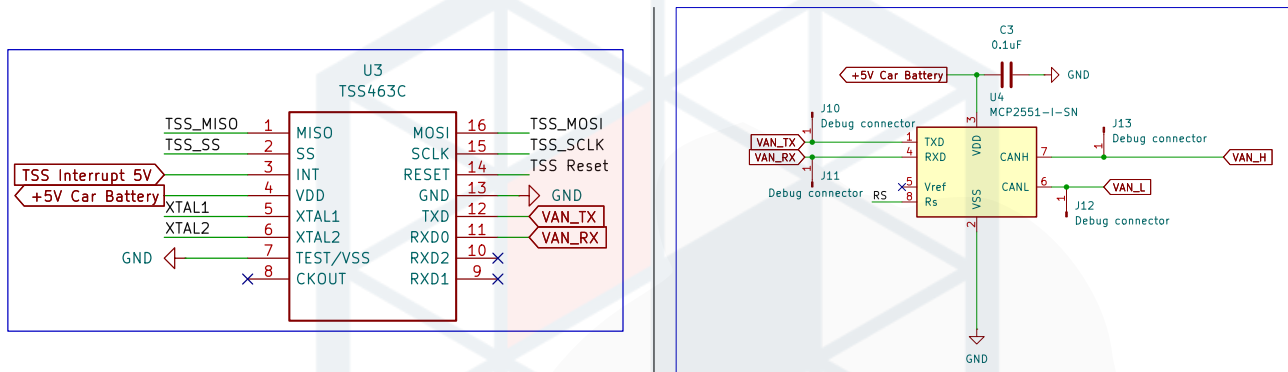
Slika 9: TSS463C and MCP2551 in the schematic
