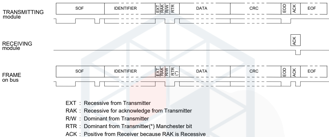
Slika 5: Normal frame transimssion with ACK
