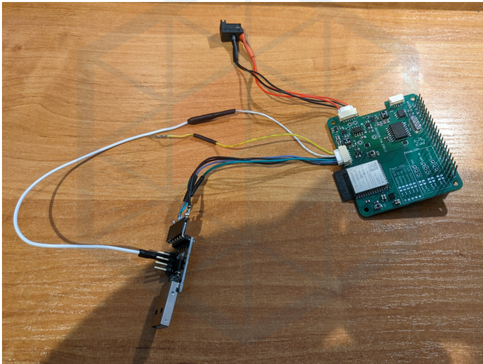
Slika 1: The gateway module setup for development
