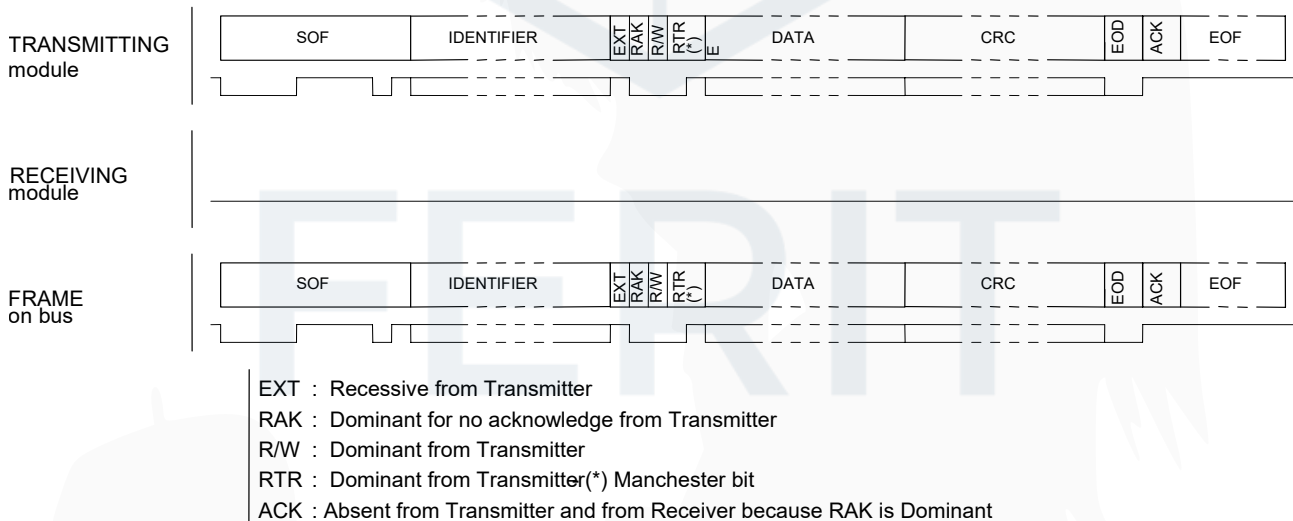
Slika 6: Normal frame transimssion without ACK
