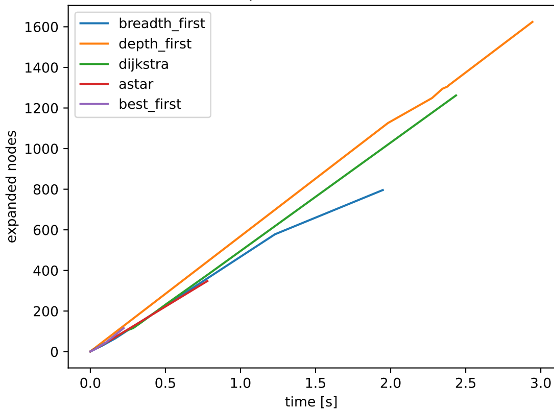
time vs expanded nodes for Planner
