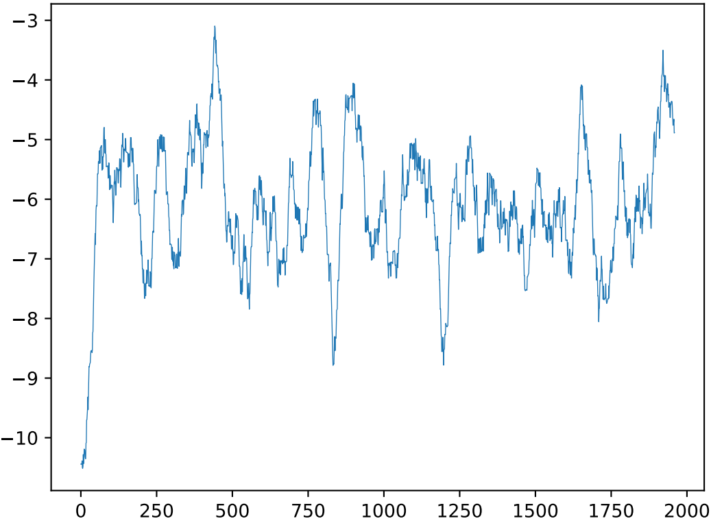
Sum of rewards for each episode (non decreasing epsilon) (average over 40
