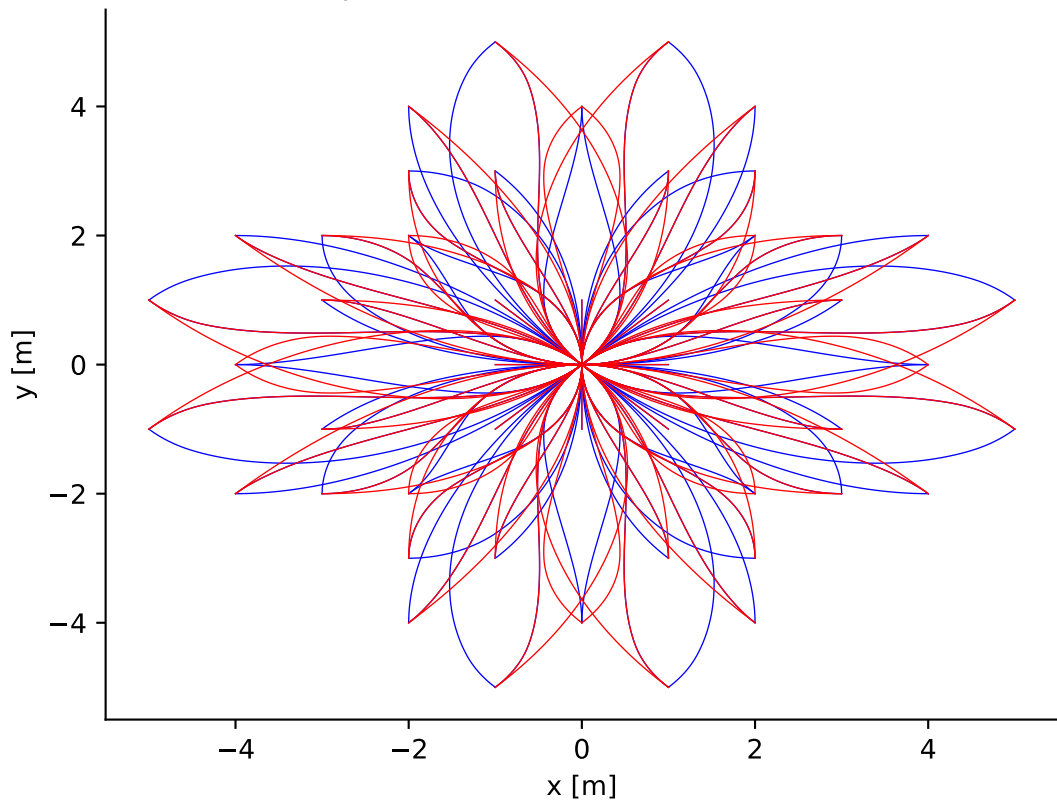
Motion primitives (forward blue, reverse red)
