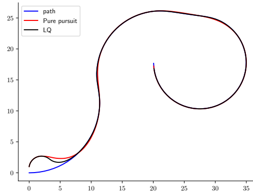
Figure 1: Sample controller performance for pure-pursuit and state-feedback (LQ) controller.
