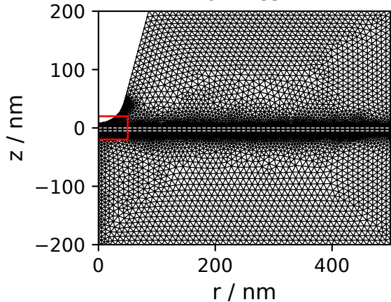
Full Mesh
