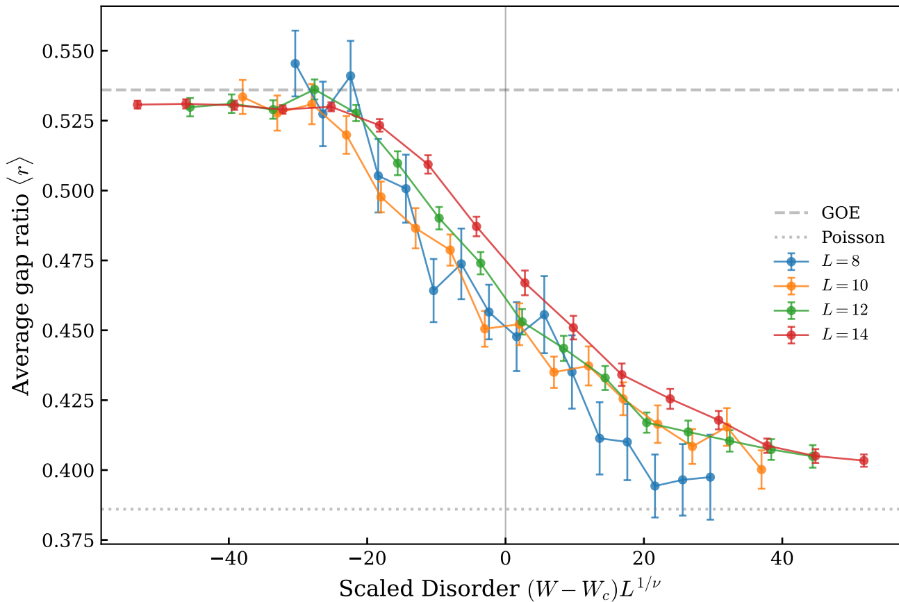
Scaling Collapse ( W_c = 4.3, \nu = 1.0 )
