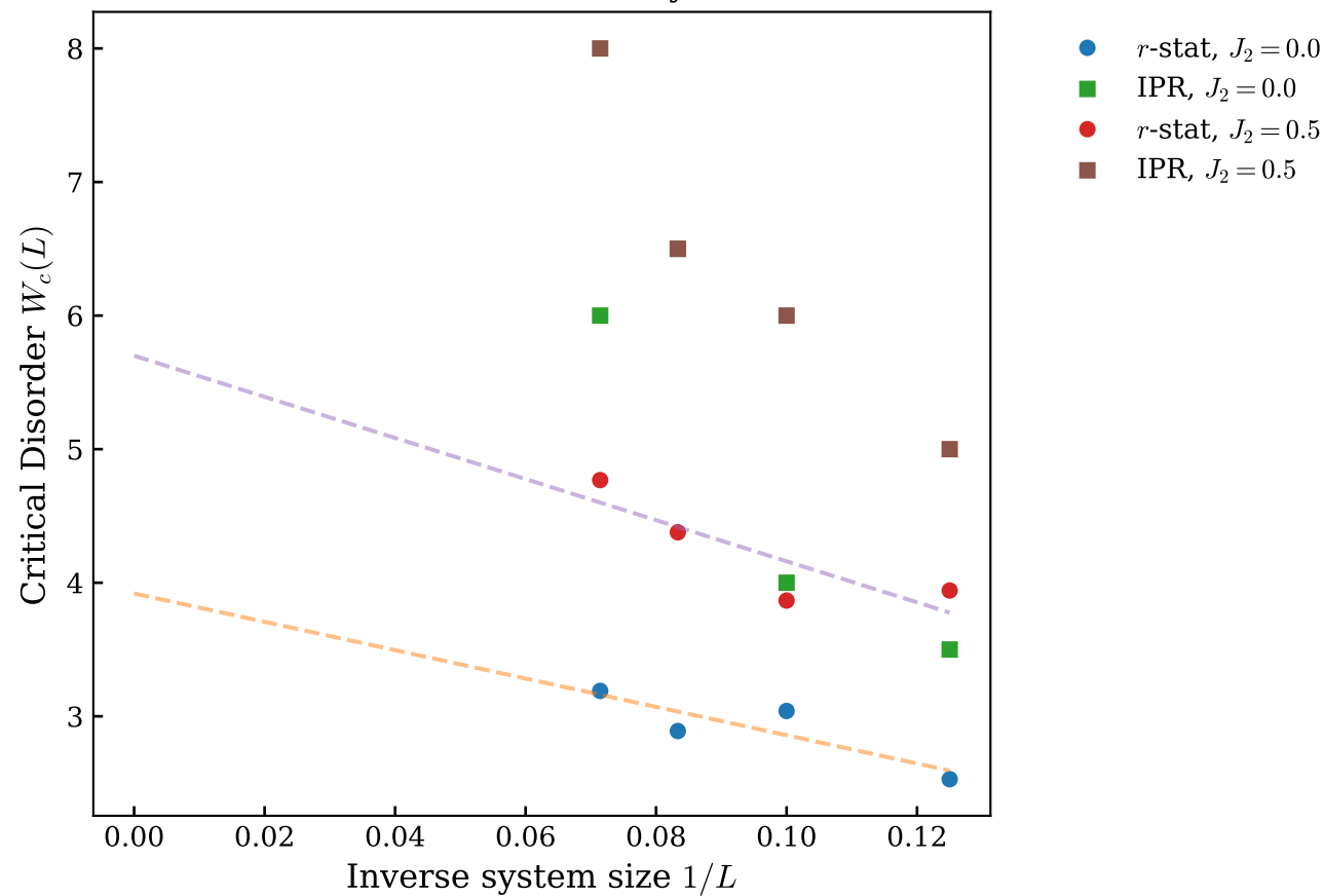
Finite-Size Drift to Thermodynamic Limit
