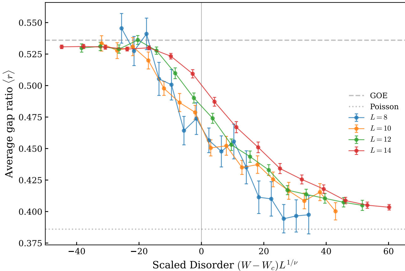
Scaling Collapse ( W_c = 3.7, \nu = 1.0 )
