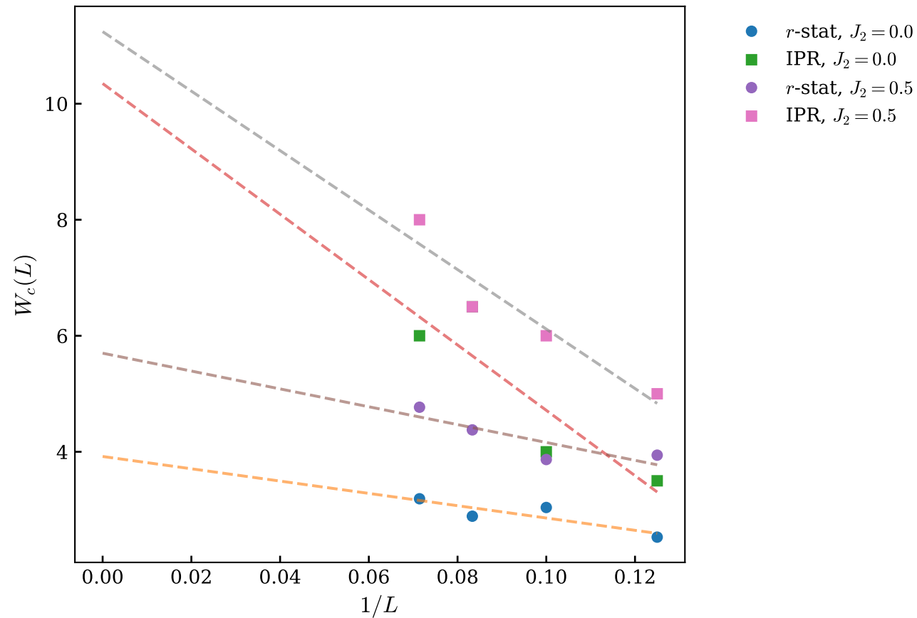
Finite-size drift and thermodynamic extrapolation of W_c
