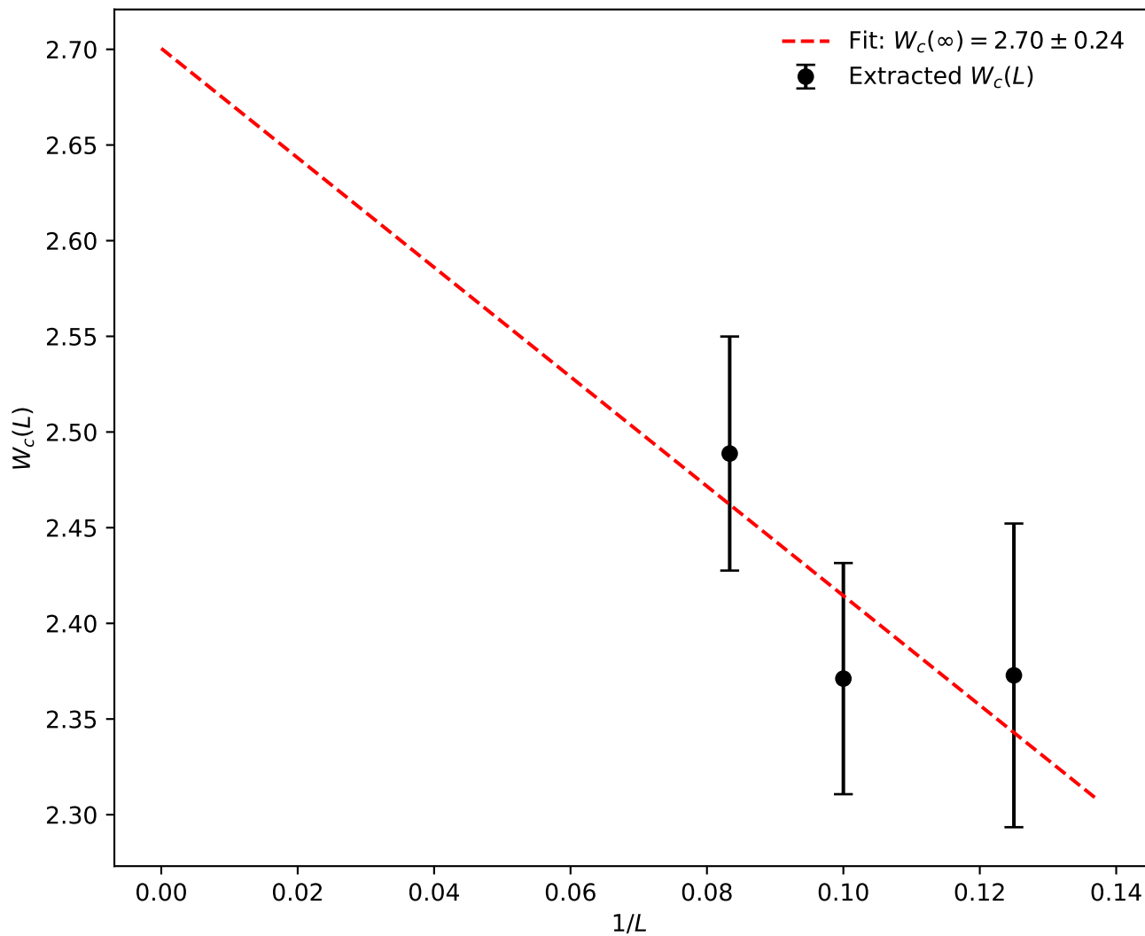
Finite-Size Scaling ( \beta_2 = 0.5 )
