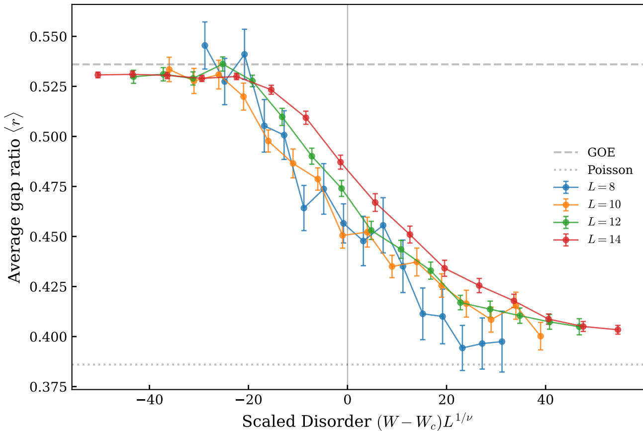
Scaling Collapse ( W_c = 4.1, \nu = 1.0 )
