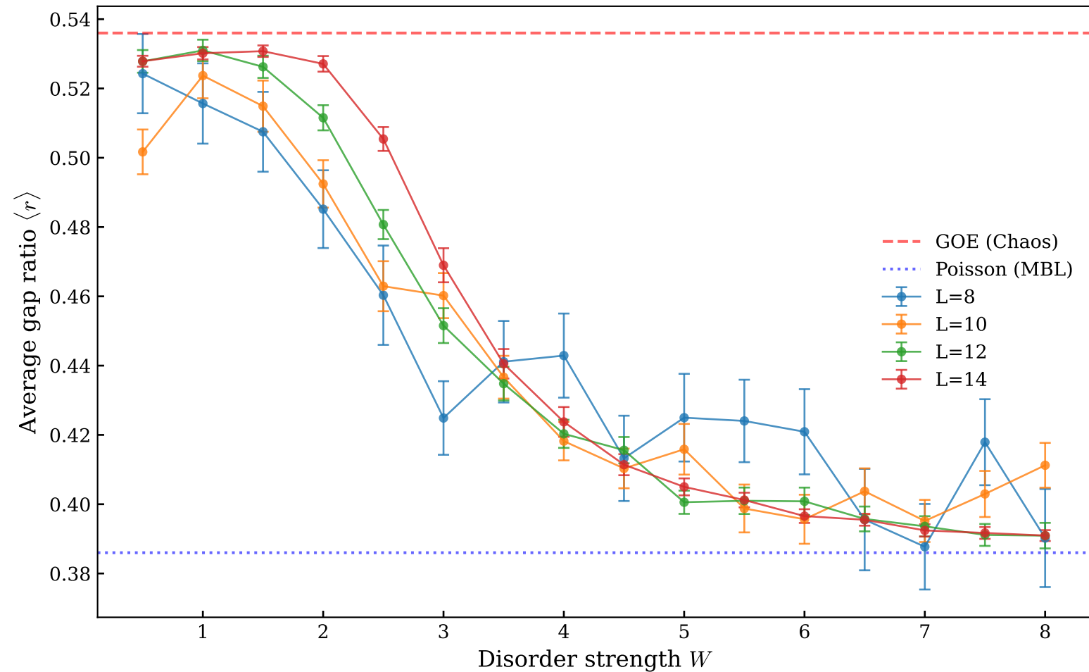
Spectral Statistics: Transition to MBL ( J_2 = 0.0 )
