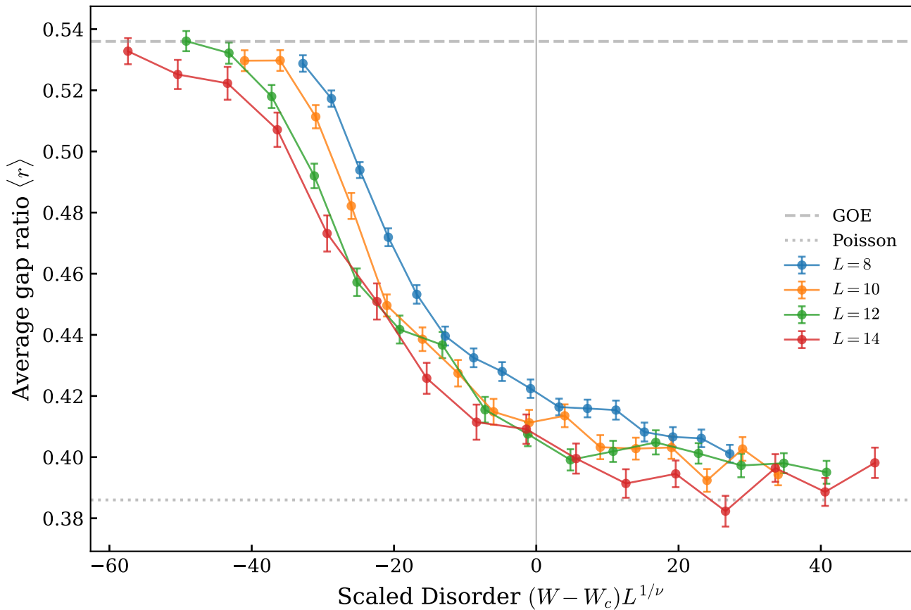
Scaling Collapse ( W_c = 4.6, \nu = 1.0 )
