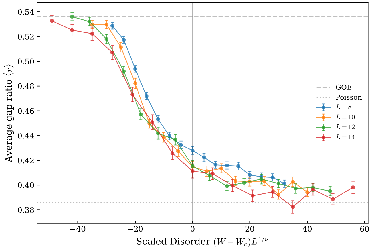
Scaling Collapse ( W_c = 4.0, \nu = 1.0 )
