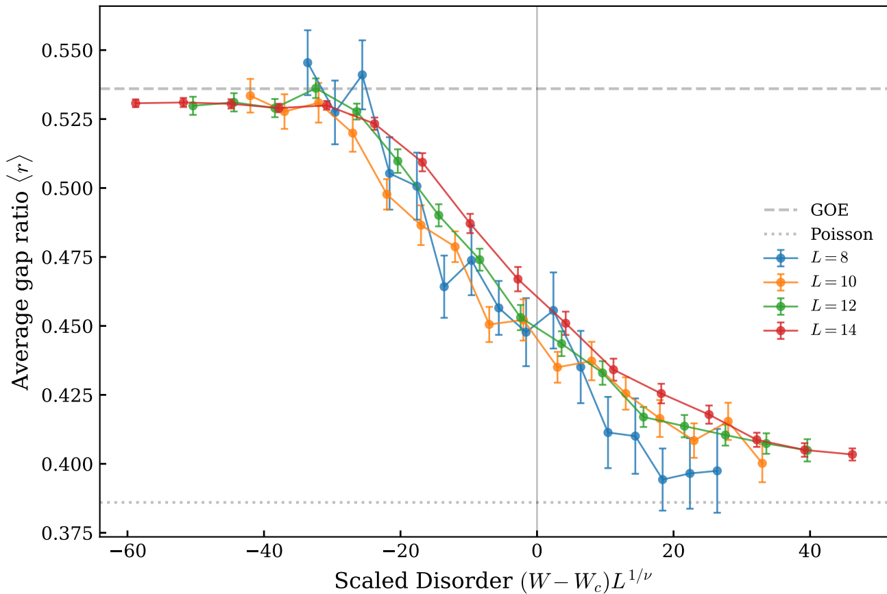
Scaling Collapse ( W_c = 4.7, \nu = 1.0 )
