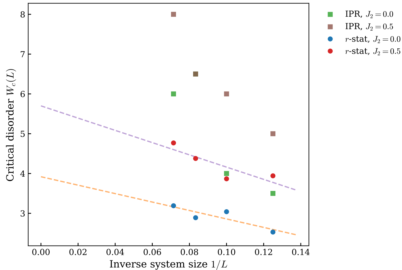
Finite-size drift of MBL transition
