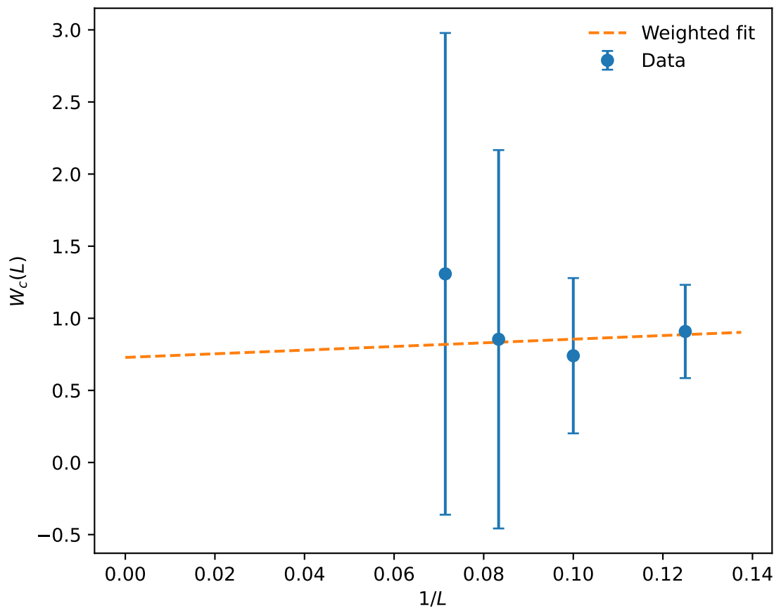
r -stat Scaling, J_2 = 0.5
