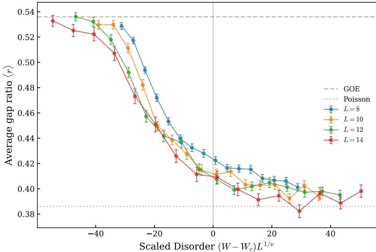
Scaling Collapse ( W_c = 4.4, \nu = 1.0 )
