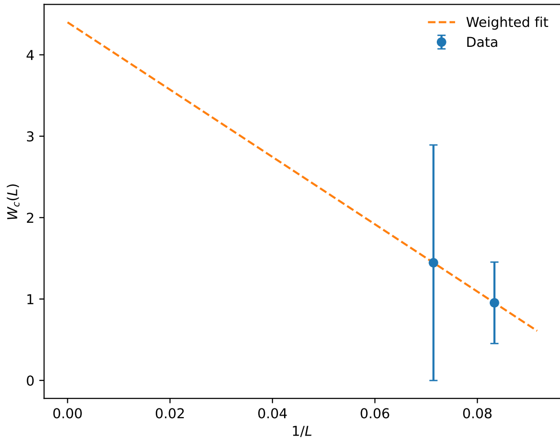
r -stat Scaling, J_2 = 0.0
