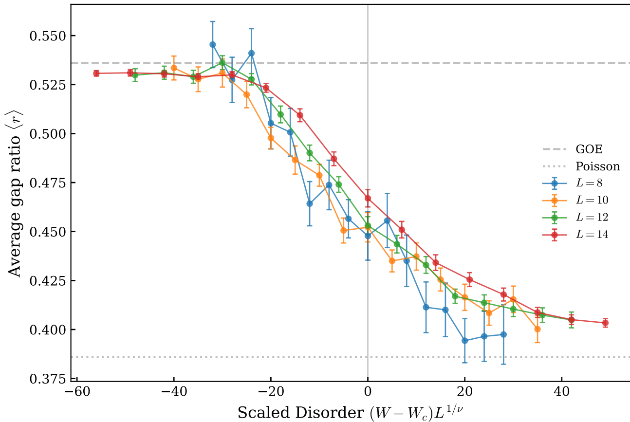
Scaling Collapse ( W_c = 4.5, \nu = 1.0 )
