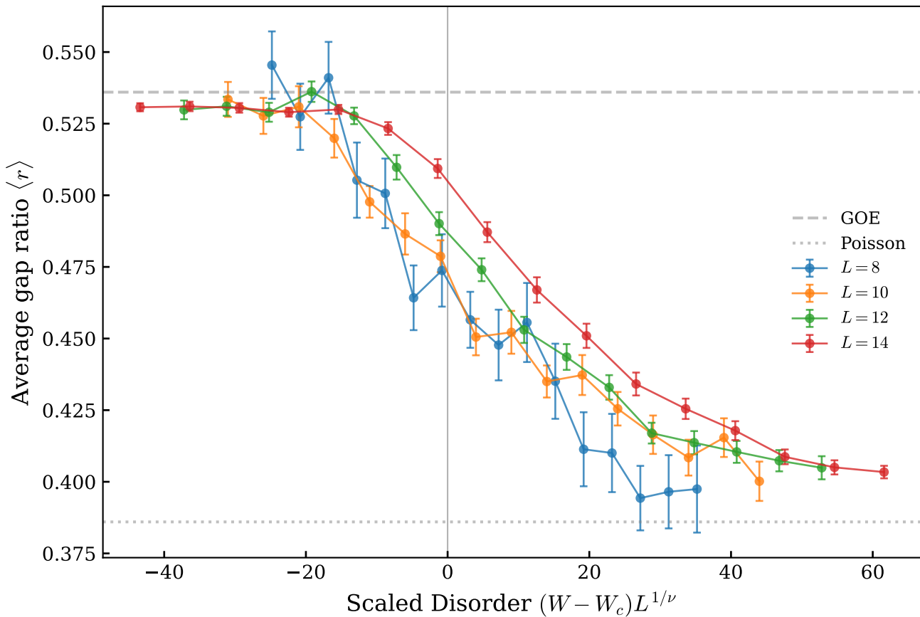
Scaling Collapse ( W_c = 3.6, \nu = 1.0 )
