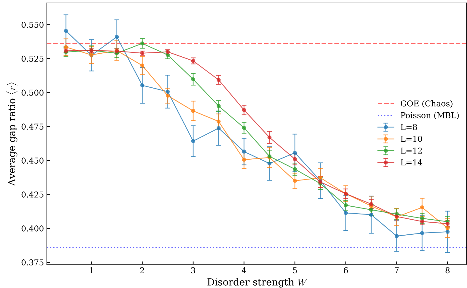
Spectral Statistics: Transition to MBL ( J_2 = 0.5 )
