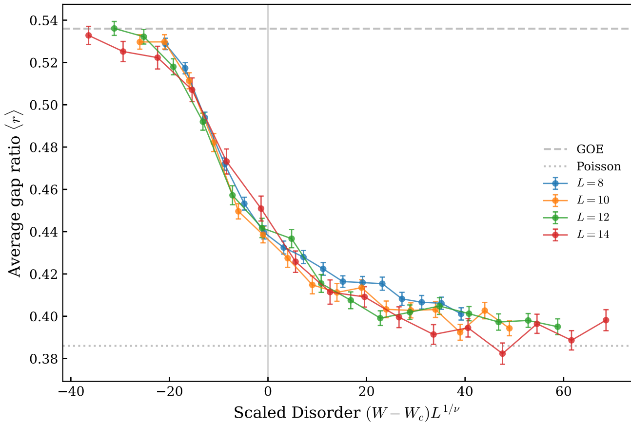
Scaling Collapse ( W_c = 3.1, \nu = 1.0 )
