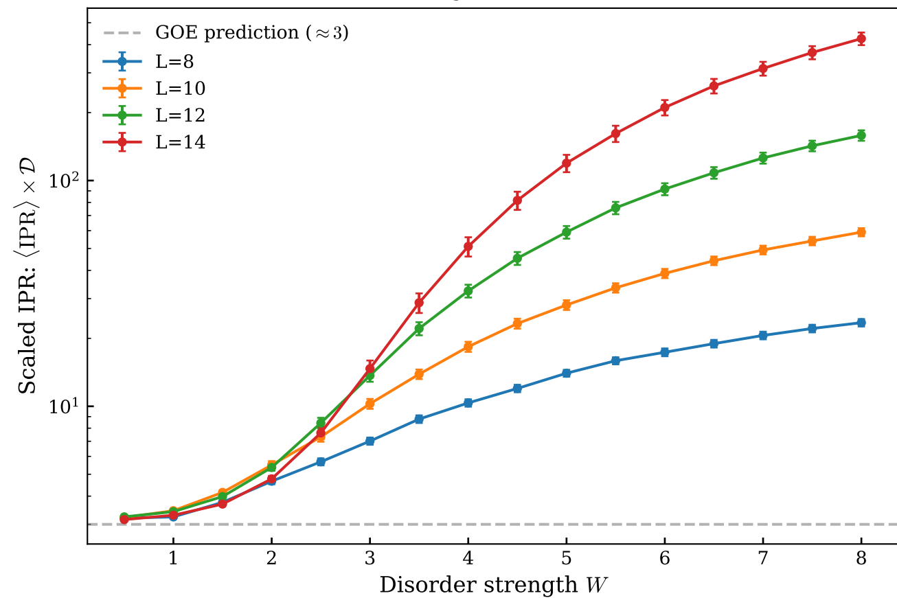
ETH Diagnostic ( J_2 = 0.5 )
