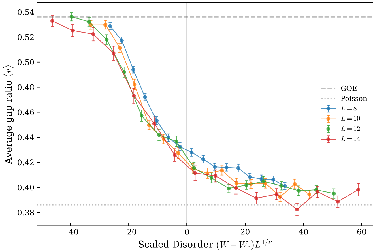
Scaling Collapse ( W_c = 3.8, \nu = 1.0 )
