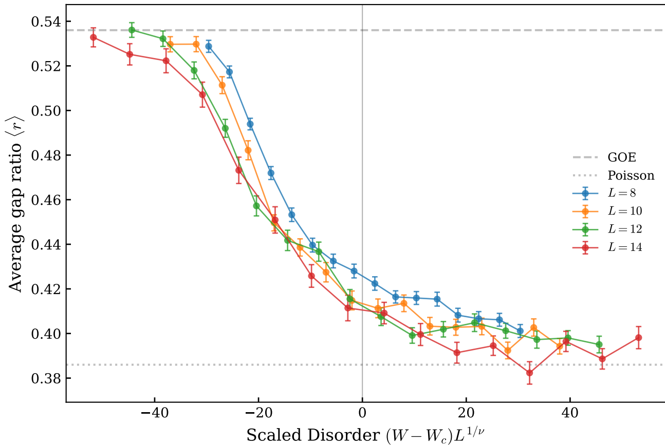
Scaling Collapse ( W_c = 4.2, \nu = 1.0 )
