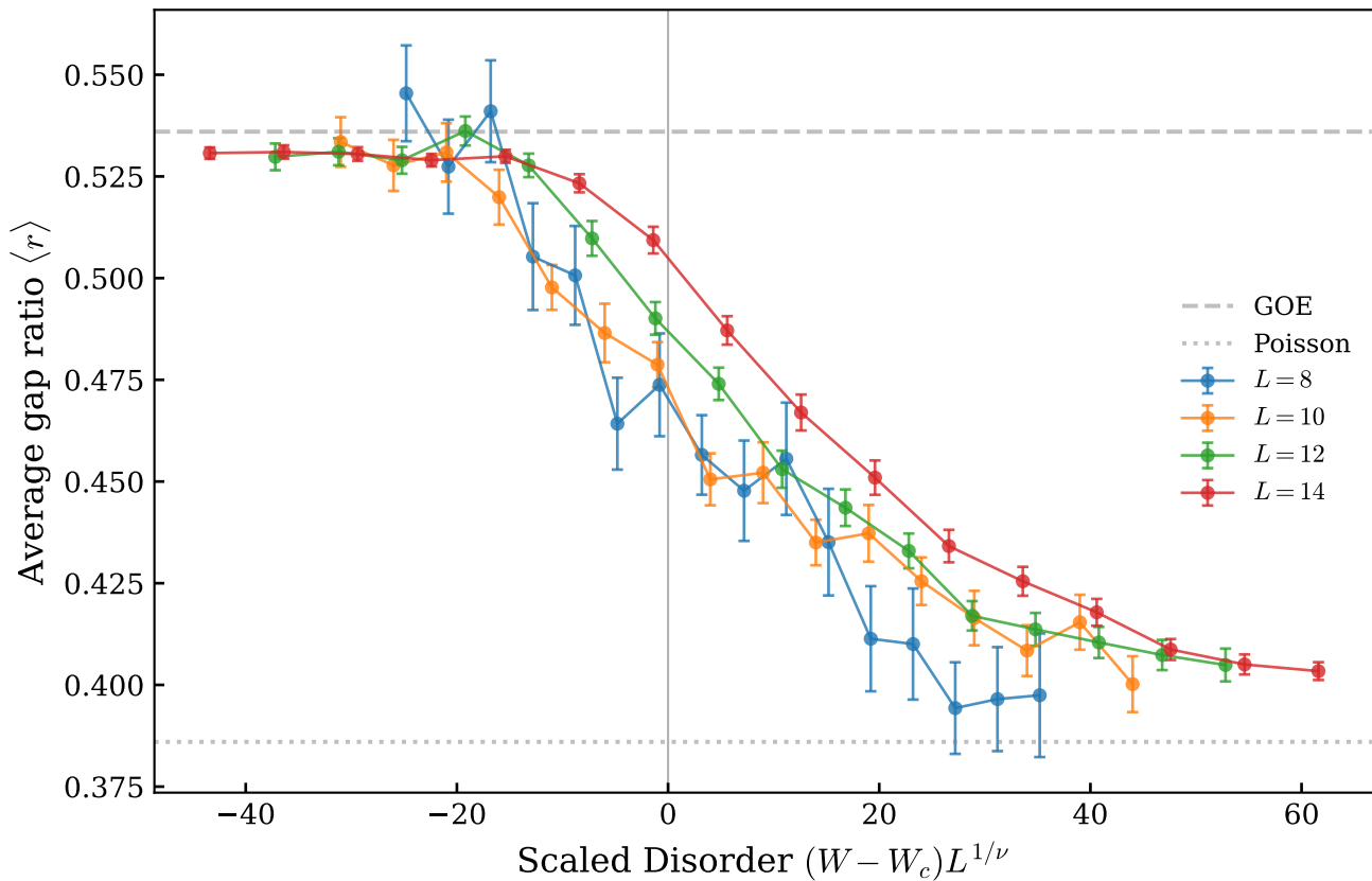
MBL Scaling Collapse ( W_c=3.6 , u=1.0 )
