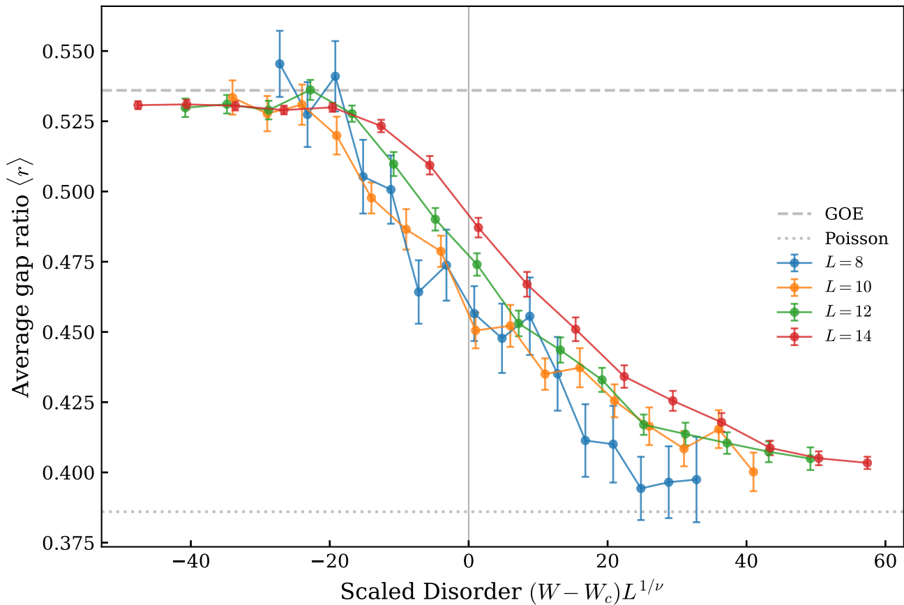
Scaling Collapse ( W_c = 3.9, \nu = 1.0 )
