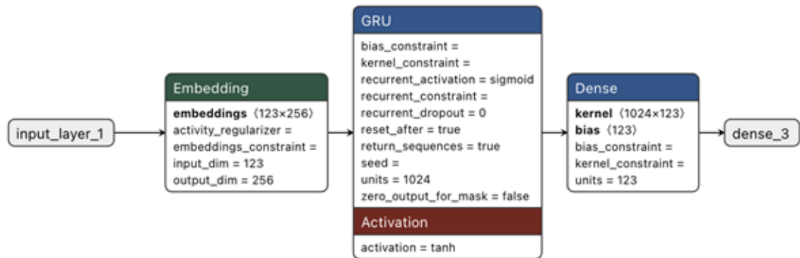
Model: "sequential_4"
