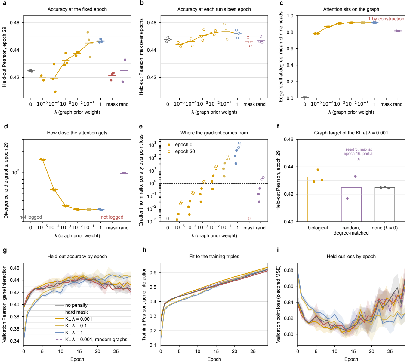
Figure 1: The sweep at three seeds per arm, read from W&B by experiments/025-solid-growth/scripts/graph_reg_sweep_readout.py . Colors name arms throughout: gray no penalty, orange the prior toward the biological graphs at \lambda \leq 10^{-2} , yellow \lambda = 10^{-1} , blue \lambda = 1 , red the hard mask ( mask ), purple the prior toward degree-matched random graphs at 10^{-3} ( rand ). (a) Held-out Pearson on the 37,673 validation triples at epoch 29, each complete seed a point, the arm mean a bar, a line through the ladder's means. (b) The same at each run's max over epochs, every run. (c) Edge recall at degree at epoch 29, mean over the nine heads. (d) Divergence of layer-1 attention from the nine graphs at epoch 29, validation pass, log scale; not computed by the model at \lambda = 0 or under the mask. (e) Gradient norm of the penalty over that of the point loss on the probe batch, epoch 0 filled and epoch 20 hollow, log scale; the two arms without a penalty are at 0. (f) The random-graph control at \lambda = 10^{-3} : arm means as bars, complete seeds as points, the running seed's max so far as a cross. (g) Validation Pearson, (h) training Pearson and (i) validation point loss by epoch, mean over complete seeds with a \pm sd band.
