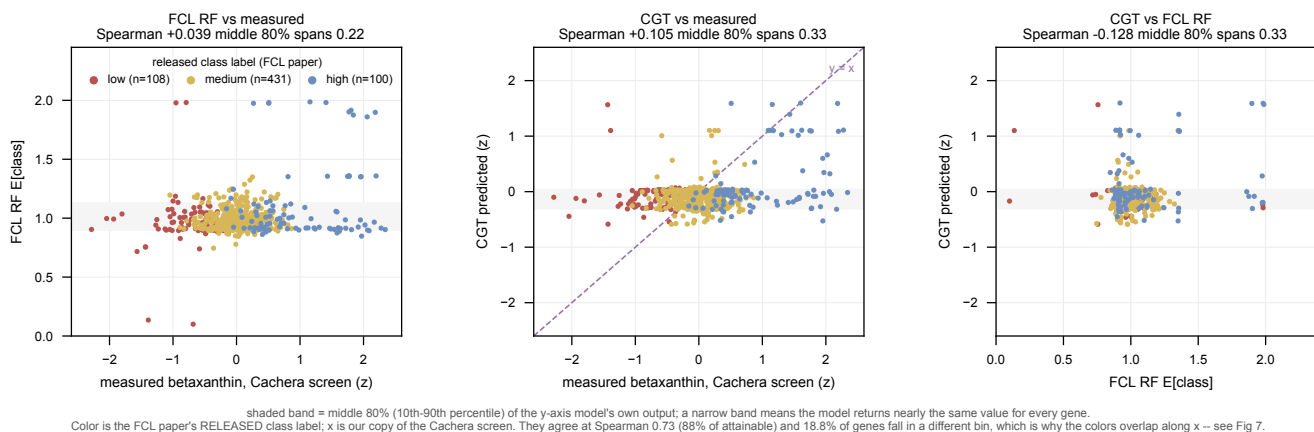
Fig 1. Both models emit a nearly constant value; the two disagree about which genes. 80 % of FCL’s genes fall inside an E[class] band of 0.22 on a 0-2 scale, 80 % of CGT’s inside 0.33 z-units. CGT’s prediction is drawn on the MEASUREMENT’s own scale (both are z-scored betaxanthin), so the middle panel shows the compression directly: the cloud is a flat band far below the y = x perfect-prediction line rather than tracking it. Colour is the FCL paper’s released class label, x is OUR copy of the same screen.
