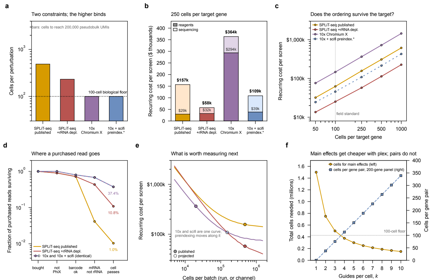
Figure 12: Six views of one decision: which platform to run. Color is the platform in every panel and only ever the platform, so the key is learned once; where a panel needs a second dimension it uses lightness within the platform's own color, or hatching against white. The asterisk marks the projected row, drawn inside the panels because a screenshot loses a caption. All four columns are 6,000 target genes in one environment at UIUC rates; panels (a), (b), (d) and (e) are priced at 250 cells per target gene. (a) Cells per perturbation, under two independent constraints (section 4.3): the depth requirement, i.e. how many cells it takes to accumulate 200,000 pseudobulk UMIs at each platform's per-cell yield, against the 100-cell biological floor below which cell-cycle and metabolic state are not averaged out. The taller bar binds, and the floor binds for every deeper platform, so past a few hundred UMIs per cell the design is limited by how many cells must be observed rather than by how deeply each is read. The preindexed column is identical to the 10x column here, which is the point of showing it: preindexing buys cells per dollar, not UMIs per cell, and is invisible to every statistical panel in this document (fig. 10d). (b) Where the recurring money goes , split into the two terms that carry the message: the platform's own color for reagents – barcoding, library preparation and, for the split-pool columns, sublibrary preparation – and its pale companion for sequencing. Sublibrary prep sits inside the reagent term rather than being drawn separately, which is how table 16 groups the same money and is also the only legible choice: at $2,970 of a $156,670 screen it is under 2% of a bar, and a band four points tall cannot carry a pattern. The dominant term moves : sequencing is 81% of split-pool spend, while for 10x it is 19% and library preparation 81%, because a genome-scale screen consumes 137 channels at $2,143 each. These are different cost structures, and an optimization that helps one (rRNA depletion, worth ~$99,000 here) does nothing for the other. Preindexing takes the 137 channels to 18 and the column to $109k, and in doing so moves that platform's dominant term onto sequencing as well – reagents 36%, sequencing 64% – but with no rRNA left to deplete. (c) Whether the ordering survives a change of target. Panel (b) prices one design; this sweeps 50 to 1,000 cells per target gene. The ordering is stable across the whole range, so the platform choice is not an artifact of the 250-cell point, and the vertical rule marks the 100-cell field standard the recommendation is actually made at. (d) What happens to a purchased read , stage by stage, and this is where the reagent comparison and the cost comparison part company. Split-pool reagents are ~22× cheaper per cell than droplet and it still loses end to end; the reversal is entirely here. Of 100 reads bought for a split-pool run, 28 are lost to the PhiX spike (10%) and to barcodes that do not resolve (a further 20% of what remains), 94 of the remainder are ribosomal, and three quarters of the cells they came from are then discarded – 1.0 read in 100 survives all four tolls. Depletion takes that to 10.8, and both droplet columns reach 37.4. The two droplet lines coincide exactly at every stage , which is worth seeing: preindexing touches no term in this panel. (e) What is worth measuring next. Every platform here has exactly one number that is both uncertain and load-bearing, and for all of them it is the same field – cells barcoded per protocol run, or cells recovered per channel – so they share an axis. 10x and scifi are one curve, and preindexing is a move along it rather than a move to a different one. (f) What multiplexing buys as guides per cell k rises. Left axis: total cells needed to hold main-effect precision across 6,000 genes falls as 1/k , from 1.5M cells at k = 1 to 0.15M at k = 10 , because every cell reports on k genes at once. Right axis: what that same cell budget delivers for one named gene pair if the library is restricted to a 200-gene panel, which grows roughly linearly in k and crosses the 100-cell floor near k = 4 . Generated by experiments/019-perturb-seq-costing/scripts/plot_economics.py , which fails rather than writing the figure if any two labels in it collide.
