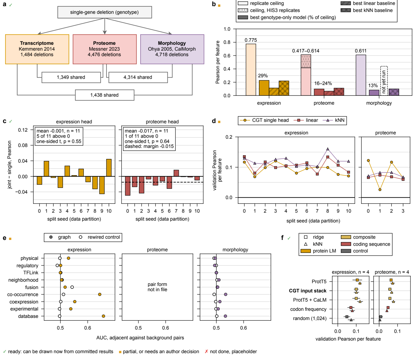
Figure 2: From the deletion alone the model reaches 13 to 29% of the replicate ceiling, and the best nearest-neighbor baseline is within 0.01 of it on expression and above it on the proteome and morphology. a, b, As fig. 1a and b. Ready; partial. c, Round v19, joint arm minus single-head arm per split seed: difference of the mean validation Pearson per feature over the registered window (expression epochs 1,000 to 1,200, proteome 200 to 400), an unselected statistic. 11 of 12 split seeds, each a different train, validation and test partition with one initialization seed; 1,099 to 1,108 training and 119 to 126 validation strains on the four seeds on file. Expression: mean -0.001 , 5 of 11 above 0, one-sided t p = 0.55 . Proteome: mean -0.017 , 1 of 11 above 0, p = 0.64 against the margin -0.015 (dashed). Neither registered test rejects. Ready; split seed 11 was unfinished. d, As fig. 1f at half width, same caveat. Partial. e, As fig. 1g at wide width. Partial. f, How much the gene representation matters to the two baselines: validation Pearson per feature, mean and s.d. over 4 split seeds, of the ridge baseline (squares) and the nearest-neighbor baseline (triangles), with rank and neighbor count selected on validation inside each seed. Five of 28 representations by rule, each the top of its class on the mean of the four validation means: best single language model (ProtT5), the model's input composite (bold), best other composite, codon frequency, best random control. The bold row is the study's model_stack , the concatenation fudt_upstream , calm , prot_T5_all , fudt_downstream that the v19 configuration inherits as node_embeddings . Ready.
