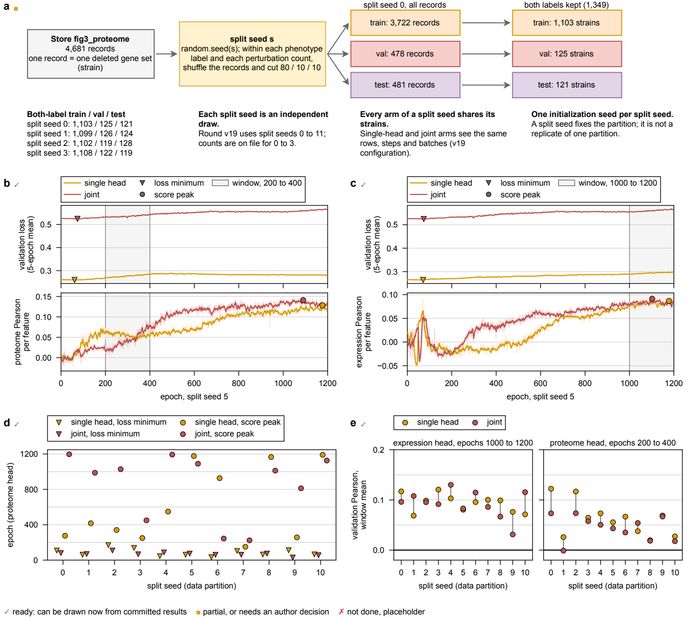
Figure 3: In round v19 the validation loss reaches its minimum before epoch 200 on every run, and the proteome score peaks later on every run. a , How a split seed becomes the strains of a run, drawn from the code. The store's 4,681 records (one record is one deleted gene set) are shuffled within each phenotype label and each perturbation count and cut 80, 10, 10 under the split seed; each side then keeps the records carrying both labels, 1,349 in all, so the both-label fractions are near and not exactly 80, 10, 10. Counts for split seeds 0 to 3. No statistic. Partial: seeds 4 to 11 are not on file. b , Proteome head, split seed 5, one run per arm: the 5-epoch centered mean of the validation loss (top) and the validation Pearson per feature (bottom; pale raw, dark its 5-epoch mean) against epoch. Triangles, loss minimum; circles, maximum of the 5-epoch mean, an upward-biased order statistic; shaded, the registered window. The joint loss sums two heads, so the two loss levels are not comparable. Split seed 5 is chosen by rule: its joint-minus-single proteome difference ( -0.012 ) is the median over the 11 complete split seeds. About 1,100 training and 125 validation strains. Ready. c , The same for the expression head of that split seed, window epochs 1,000 to 1,200. Ready. d , Proteome head, all 11 complete split seeds, 22 runs: epoch of the loss minimum (triangles) and of the score peak (circles). Ready. e , The window scores behind fig. 2c: mean validation Pearson over the registered window, single-head and joint arm, 11 split seeds, 33 runs. Unselected. Ready.
