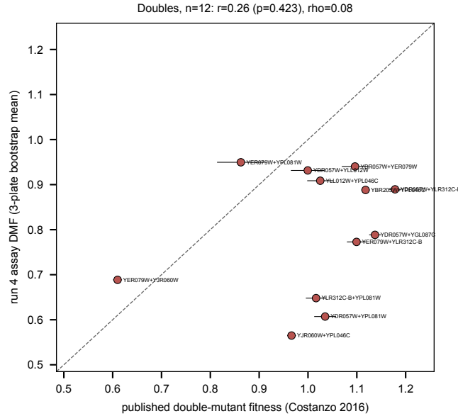
Fig. 7 Run 4 double-mutant fitness against published Costanzo DMF. The 13th double, the novel YPL046C+YPL081W, is absent because no published value exists for it.
