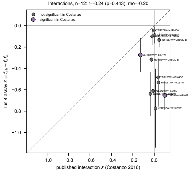
Fig. 8 Run 4 \varepsilon against published Costanzo \varepsilon , the two Costanzo-significant pairs marked. Every point sits below zero and the published spread is not recovered. This panel is published as the record of a diagnosed artifact, not as a measurement of epistasis.
