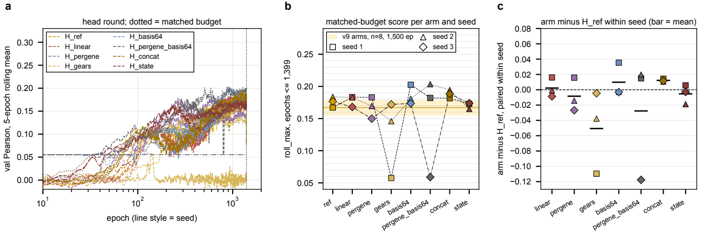
Figure 7: Only H\_concat is above H\_ref in every seed, by about 0.012, a direction three seeds cannot resolve. a, validation Pearson (5-epoch rolling mean) of all 24 runs, color by arm, line style by seed; the dotted line is the matched budget. b, roll\_max at epochs \leq 1,399 per arm and seed, lines joining one seed's arms; the band is the eight v9 long-budget arms at 1,500 epochs. c, the paired difference against H\_ref within seed, bar at the mean. Generated by head\_round\_readout.py .
