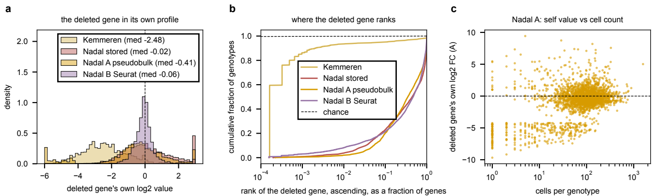
Figure 11: The deleted gene is the most reduced gene of its own profile in 60 % of Kemmeren deletions and under 1 % of Nadal-Ribelles genotypes (b). a , the deleted gene's own \log_2 value per genotype for Kemmeren and three Nadal-Ribelles statistics. b , cumulative distribution of the deleted gene's ascending rank as a fraction of genes in the profile, log axis; the dashed diagonal is chance. c , for the pseudobulk statistic, the deleted gene's own value against the cells behind the genotype; the band near -5 to -8 at low counts is the pseudocount floor of a near-empty pseudobulk. Generated by nadal_identify_deletion.py .
