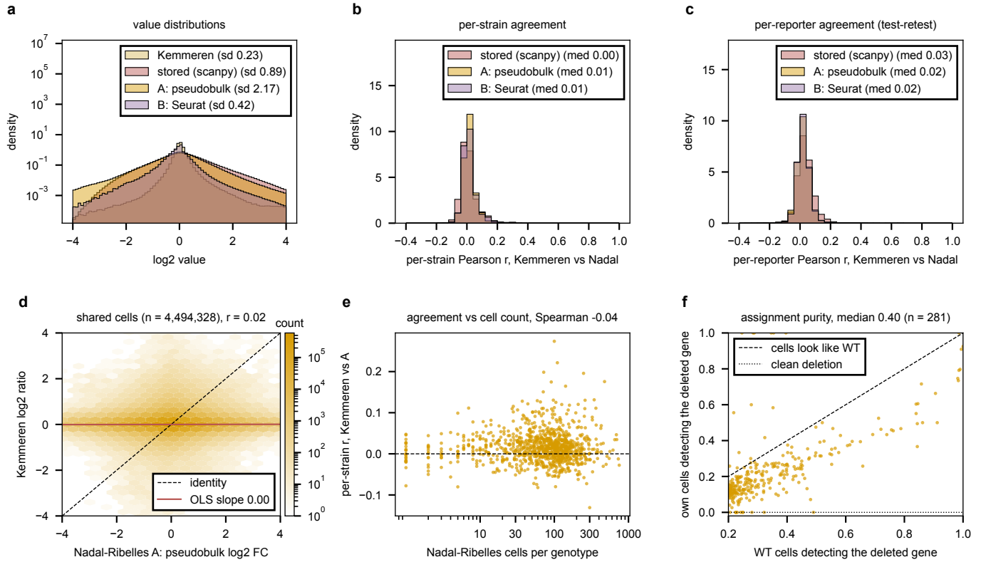
Figure 10: Recomputing the fold change from the raw cells does not recover agreement with Kemmeren (b, c), because the labeled cells are only about 40 % the genotype they carry (f). a , \log_2 values of Kemmeren and of three Nadal-Ribelles versions: as stored, the bulk-like pseudobulk ratio (A) and Seurat's avg_log2FC (B). b , per shared deletion, the Pearson across reporters with Kemmeren for each version; c , the same per reporter across shared strains. d , Kemmeren against A on every shared cell. e , per-strain agreement of A against the cells behind the genotype. f , assignment purity: for each genotype whose deleted gene wild type detects in at least a fifth of cells, the fraction of the genotype's own cells detecting that gene against the wild-type fraction; the dashed identity is what cells that are not the genotype look like, the dotted zero a clean deletion. Generated by cross_study_recomputed.py from nadal_pseudobulk_recompute.R and nadal_assignment_purity.R .
