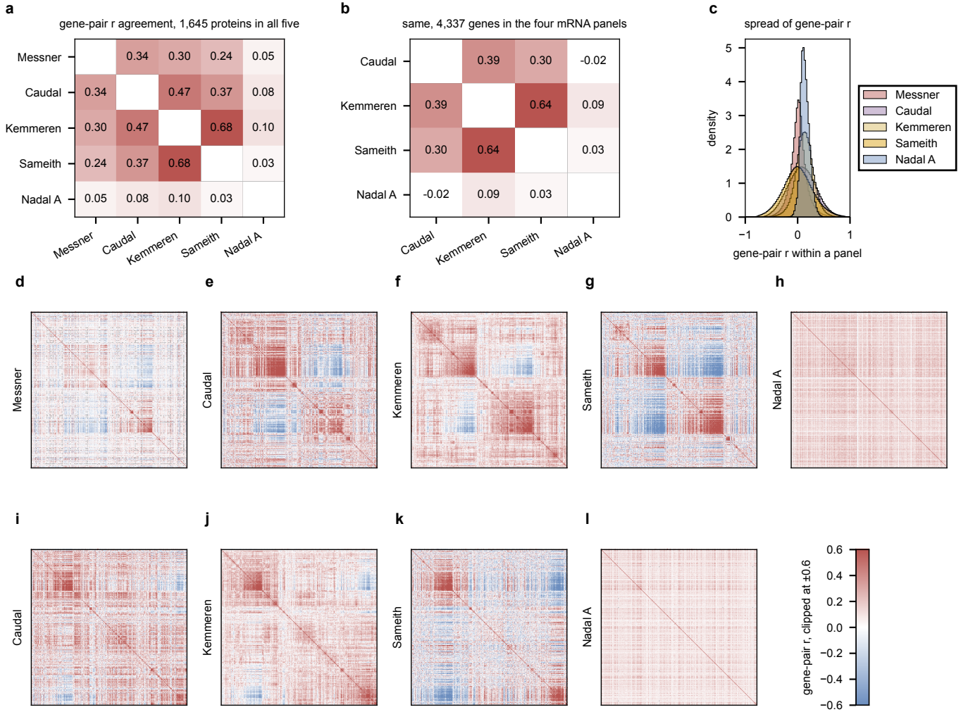
Figure 15: Four panels that differ in platform, perturbation and medium agree on which gene pairs co-vary (0.24 to 0.68, a , b ), and Nadal-Ribelles agrees with none, its matrix nearly flat ( h , l ). Within a panel, two genes get one Pearson across that panel's own strains; no strain is aligned between panels. a , Spearman between the upper triangles of two panels' gene-by-gene matrices on the 1,645 proteins measured in all five panels. b , the same on the 4,337 genes measured in the four mRNA panels. c , the distribution of the gene-pair r within each panel on the protein gene list. d–h , the five matrices on the protein gene list, and i–l the four mRNA matrices on the expression gene list, every matrix in the ordering given by average-linkage clustering of Kemmeren's matrix on that gene list, so a block in Kemmeren can be looked for at the same place in every other panel; color clipped at \pm 0.6 . Messner spans 4,549 deletions, Caudal 943 isolates, Kemmeren 1,484 deletions, Sameith 82 single deletions, Nadal-Ribelles A the 2,243 deletions with at least 50 cells. Generated by gene_covariation_all.py .
