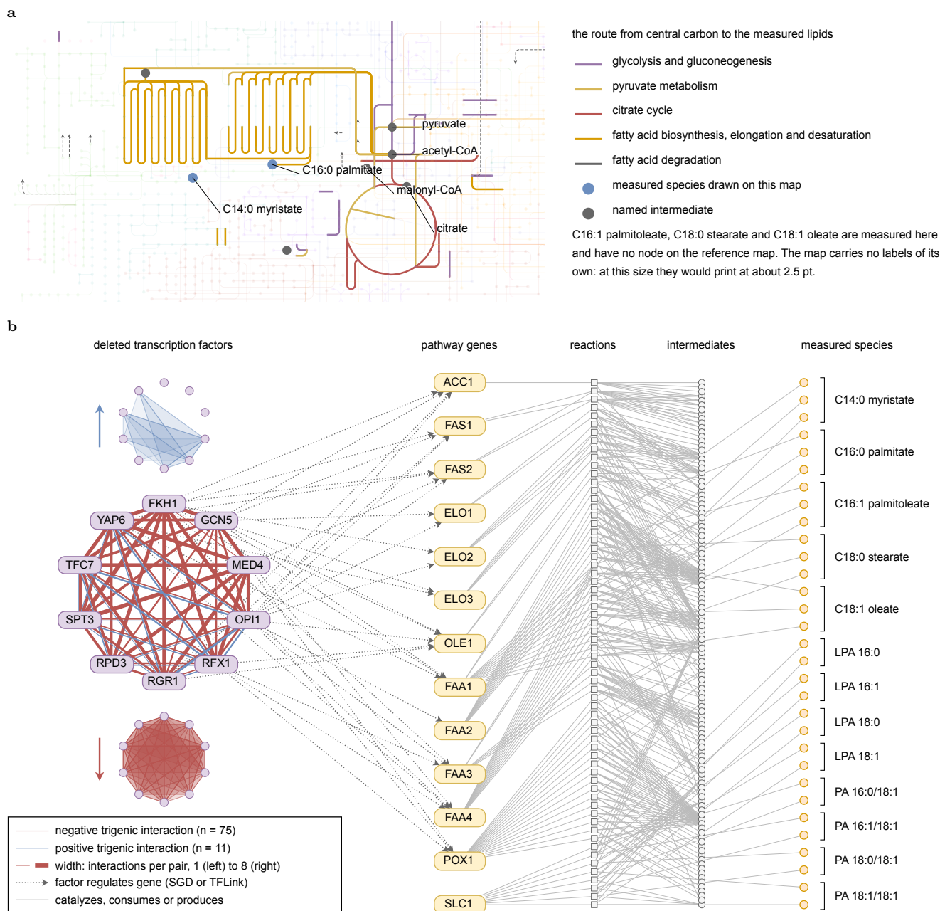
Fig. 5 Trigenic interactions on total fatty acid titer, drawn upstream of the pathway they act through. a , Where the measured chemistry sits in metabolism, on the iPath3 reference map of KEGG's global metabolic pathways. Colored are the yeast reactions of glycolysis and gluconeogenesis, pyruvate metabolism, the citrate cycle, fatty acid biosynthesis, elongation and desaturation, and fatty acid degradation, taken from KEGG's own gene lists for those pathways rather than chosen here. The two measured species the reference map carries a node for are marked, as are four named intermediates on the route; the other three measured species have no node on that map. The map's own labels are not reproduced, because at this size they would print below the minimum type size. b , The ten deleted transcription factors are arranged in a circle at left. Edges within the circle are the 86 trigenic interactions significant at a 5% false discovery rate within the total-titer readout under the multiplicative model, 75 negative (brick) and 11 positive (blue), each drawn as the three edges of its triangle; edge width is the number of interactions the pair takes part in, from 0.40 pt at 1 to 2.15 pt at 8. Every one of the 45 pairs is in at least one negative interaction, so a pair that also carries a positive one would hide it: the two signs of a pair are therefore drawn as two parallel lines, offset perpendicular to the pair by half their combined width, and neither covers the other. Above and below that circle the same ten factors are drawn again at the same angles, unlabeled, carrying only the positive interactions (blue, above) and only the negative ones (brick, below). The two shapes are what the combined circle cannot show. The negatives reach all 45 pairs and every factor, with up to 8 interactions on one pair. The positives reach 17 pairs and 7 factors, at most 4 on a pair, and FKH1, GCN5 and MED4 take part in none of them. Dotted arrows are regulatory links from a factor to a pathway gene in the SGD regulatory graph or TFLink; three of the ten factors have none. The columns to the right are the 13 core fatty acid pathway genes, the 64 reactions they catalyze, the intermediates those reactions consume or produce, and the 31 measured species, one node per compartment (peroxisome, ER membrane, lipid particle) with a bracket per species. LPA, 1-acyl-sn-glycerol 3-phosphate; PA, phosphatidate, written as the two acyl chains.
