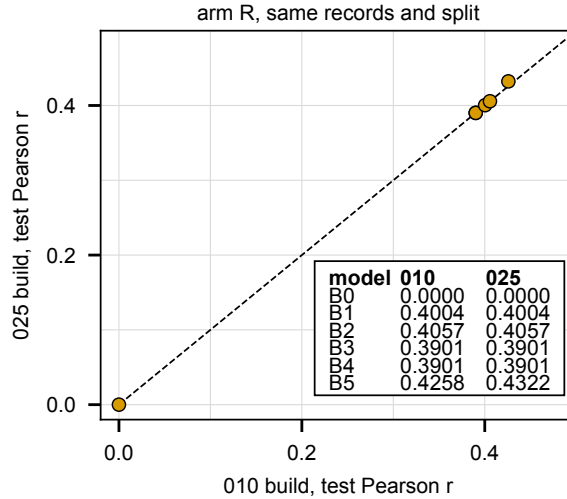
Figure 6: Arm R test Pearson on the 025 build against the same model on the 010 build. Every closed-form model lies on the identity line to numerical precision; the nonlinear baseline sits 0.006 above it, inside its own three-seed spread.
