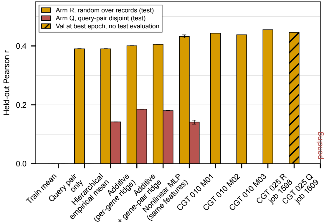
Figure 5: Held-out Pearson on the 025 build for each baseline under arm R and arm Q, with the transformer rows that exist: the three 010 checkpoints and the arm R replication. The hatched bar is a validation maximum, not a test number, and the arm Q transformer slot waits on job 1609.
