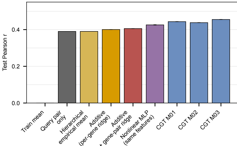
Figure 2: Test Pearson for every model. Error bars on the nonlinear baseline are the standard deviation across three seeds; the transformer bars are three separate training runs shown individually.
