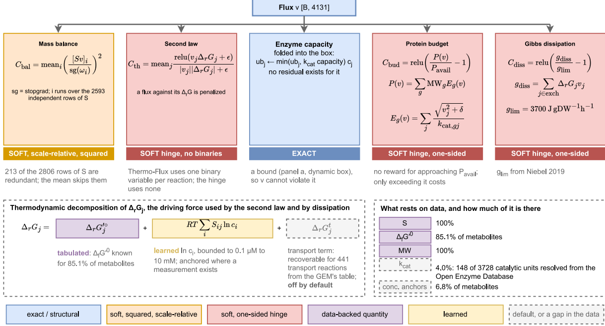
Figure 3. The flux layer, from gene tokens to a feasible flux vector and its residuals. (a) A deletion sets gene availability to zero as a hard fact, not a learned gate; complexes take a softmax over subunits and isozymes sum, and enzyme capacity enters the bounds rather than the loss, so the box holds by construction and contributes no loss term. (b) Five residuals hang off the flux. One is exact and the other four are smooth penalties, none requiring a binary variable. The insets give the three-term decomposition of the reaction driving force and the fraction of each input that is measured rather than defaulted.
