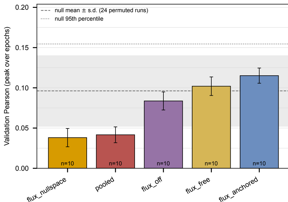
Figure 6. Every arm sits inside the noise band. Bars are the mean maximum validation Pearson for betaxanthin across ten seeds, error bars the standard error. The dashed line and shaded band are the mean and standard deviation of 24 label-permutation runs; the dotted line is their 95th percentile. No arm reaches that percentile, and the smallest p-value across all 22 configurations tested is 0.24.
