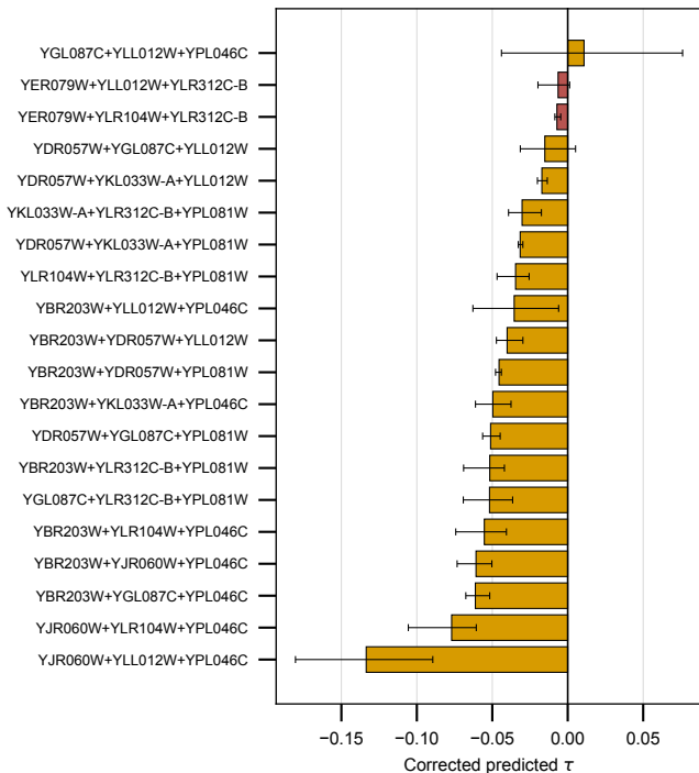
The 20 build-list triples, re-ranked red = contains an untrained gene (2)
