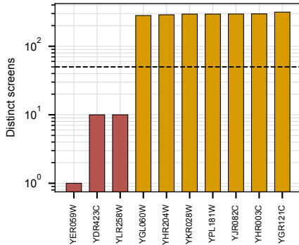
3 panel genes sit under the floor
