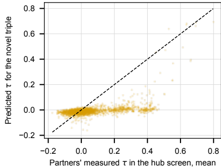
r = 0.49 over 2,730 triples
