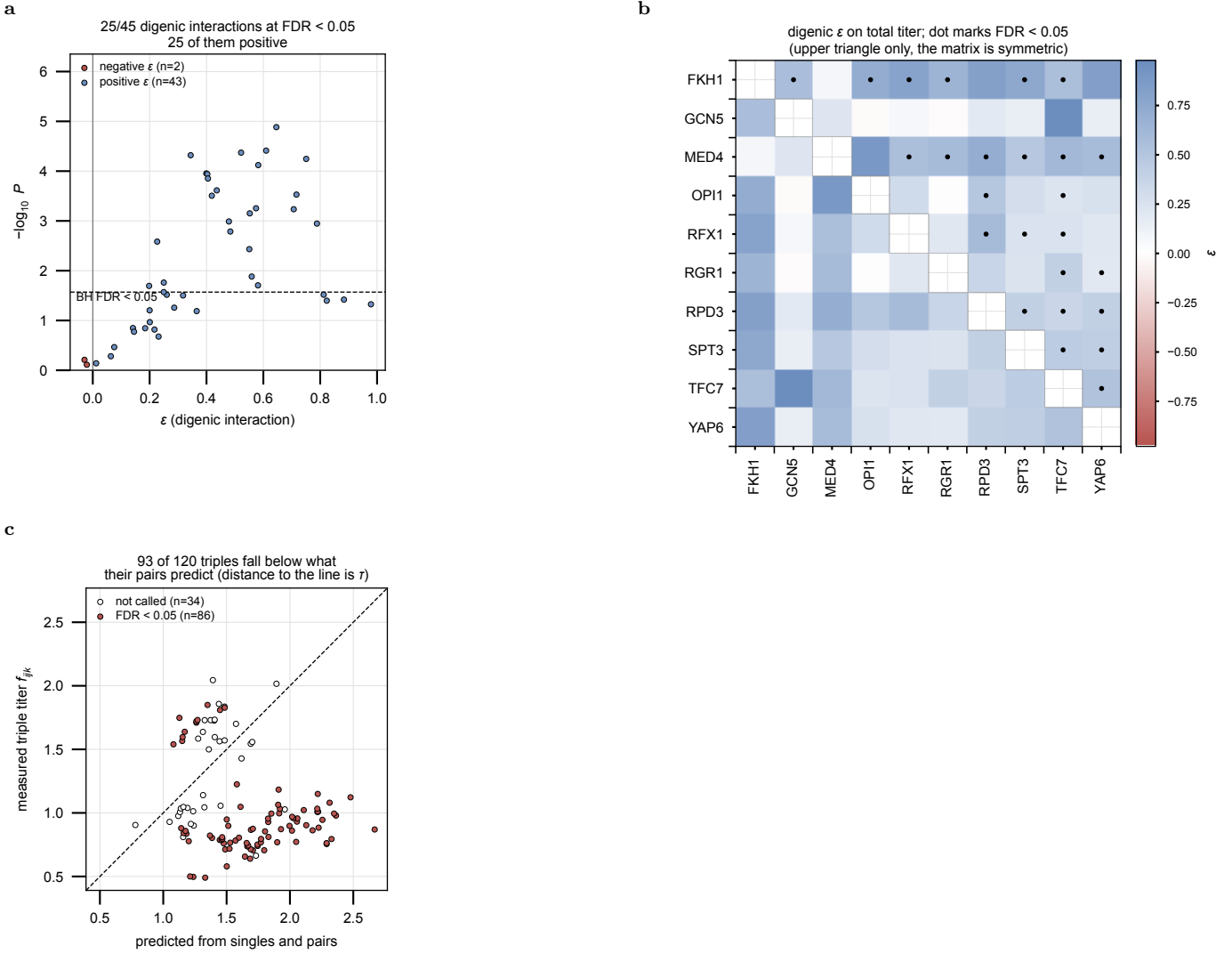
Supplementary Figure 1 The digenic layer on total fatty acid titer. a , Digenic score \varepsilon against evidence for the 45 double deletions under the multiplicative model. The dashed line marks the largest P that Benjamini-Hochberg rejects at a 5% false discovery rate over the 45 tests of this readout; 25 pairs clear it and all 25 are positive. b , Every pair's \varepsilon as a matrix over the ten factors, blue positive and brick negative on a scale centered at zero. The matrix is symmetric and the dots marking a false-discovery-rate call are drawn in the upper triangle only. c , Each triple's measured titer against the titer predicted from its singles and its pairs, f_i f_j f_k + \varepsilon_{ij} f_k + \varepsilon_{ik} f_j + \varepsilon_{jk} f_i . The vertical distance to the diagonal is the trigenic score \tau , so a point below the line is a triple that produces less than its own pairs predict; 93 of 120 do. Filled points are triples called at a 5% false discovery rate within total titer.
