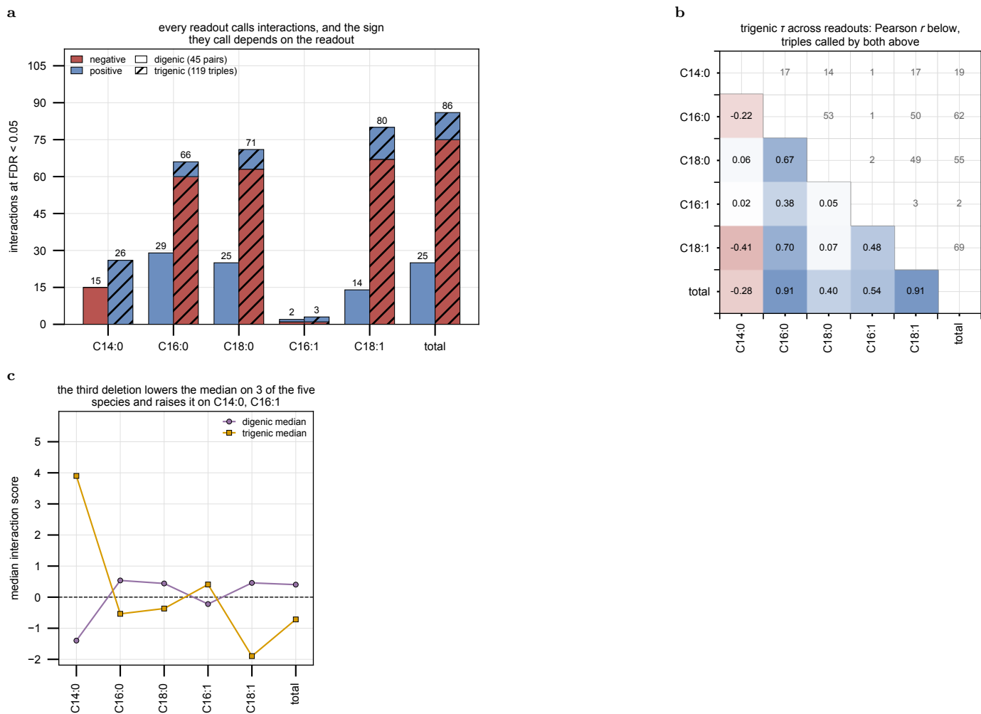
Supplementary Figure 2 The five measured species behind the summed total. a , Interactions called at a 5% false discovery rate within each readout, digenic (solid) and trigenic (hatched), stacked by sign, blue positive and brick negative. Counts above each bar are the totals. b , Trigenic \tau compared across readouts over the same 119 triples: Pearson r below the diagonal, and above it the number of triples called at a 5% false discovery rate in both readouts. c , Median interaction score per readout for both orders. The gap between the two lines is the quantity the main text reports on total titer, and its sign is not the same on every species.
