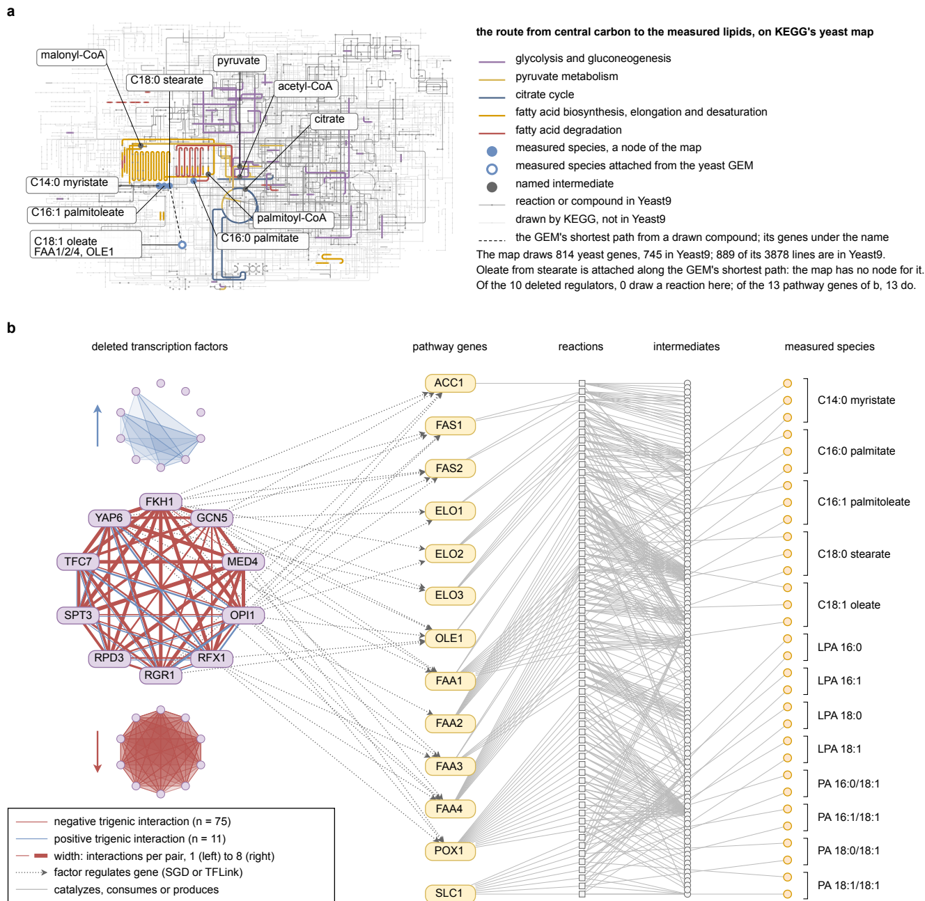
Fig. 5 Trigenic interactions on total fatty acid titer, drawn upstream of the pathway they act through. a , Where the measured chemistry sits in metabolism: KEGG's global map of yeast metabolism, redrawn as vector from the coordinates KEGG publishes for it, with the yeast genome-scale model overlaid. Reactions and compounds the model contains are drawn in gray; what KEGG draws but the model lacks is fainter. The map places 814 yeast genes, 745 of them in the model, and 889 of its 3,878 reaction lines; the model's transport, exchange and per-chain lipid reactions have no place on any such map and are the part panel b carries. Colored are the yeast reactions of glycolysis and gluconeogenesis, pyruvate metabolism, the citrate cycle, fatty acid biosynthesis, elongation and desaturation, and fatty acid degradation, taken from KEGG's own gene lists for those pathways rather than chosen here. A gene on more than one list takes the first in the order central carbon, degradation, biosynthesis, which is what keeps the degradation arm visible: KEGG lists POX1, the acyl-CoA oxidase this chassis deleted, with the unsaturated fatty acids too. Filled blue nodes are the four measured species the map draws; gray nodes are five named intermediates on the route. Oleate has no node on the map, as the free acid or as oleoyl-CoA, and is attached as an open ring along the shortest path of the same genome-scale model from stearate, with the genes of that path under its name. Of the ten deleted regulators, none is among the genes the map draws, which is the point of the panel: the deletions act on metabolism from outside it. All thirteen pathway genes of panel b are drawn. The map's own labels are not reproduced, because at this size they would print below the minimum type size. b , The ten deleted transcription factors are arranged in a circle at left. Edges within the circle are the 86 trigenic interactions significant at a 5% false discovery rate within the total-titer readout under the multiplicative model, 75 negative (brick) and 11 positive (blue), each drawn as the three edges of its triangle; edge width is the number of interactions the pair takes part in, from 0.40 pt at 1 to 2.15 pt at 8. Every one of the 45 pairs is in at least one negative interaction, so a pair that also carries a positive one would hide it: the two signs of a pair are therefore drawn as two parallel lines, offset perpendicular to the pair by half their combined width, and neither covers the other. Above and below that circle the same ten factors are drawn again at the same angles, unlabeled, carrying only the positive interactions (blue, above) and only the negative ones (brick, below). The two shapes are what the combined circle cannot show. The negatives reach all 45 pairs and every factor, with up to 8 interactions on one pair. The positives reach 17 pairs and 7 factors, at most 4 on a pair, and FKH1, GCN5 and MED4 take part in none of them. Dotted arrows are regulatory links from a factor to a pathway gene in the SGD regulatory graph or TFLink; three of the ten factors have none. The columns to the right are the 13 core fatty acid pathway genes, the 64 reactions they catalyze, the intermediates those reactions consume or produce, and the 31 measured species, one node per compartment (peroxisome, ER membrane, lipid particle) with a bracket per species. LPA, 1-acyl-sn-glycerol 3-phosphate; PA, phosphatide, written as the two acyl chains.
