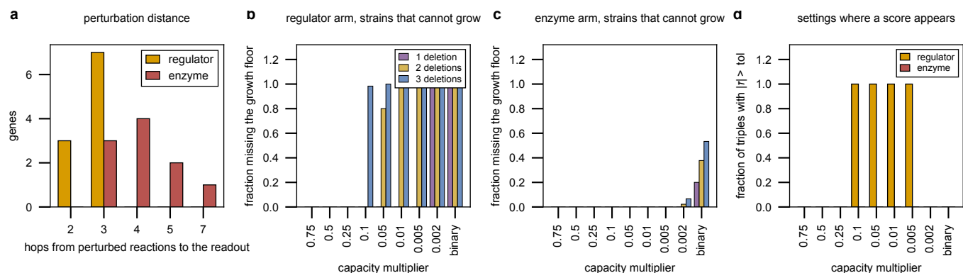
Supplementary Figure 3 A minimal flux model does not settle the regulator-against-enzyme comparison. a , Distance from the perturbed reactions to the five readout exchanges, counted in reactions on the model's reaction-metabolite graph with currency metabolites dropped. The regulator arm is closer than the enzyme arm, not further, because a regulator's reaction set is the union over hundreds of targets. b , c , The fraction of combinations at each order that miss the growth floor and export nothing, per capacity multiplier. In the regulator arm this is where every nonzero interaction score comes from. d , The fraction of the 120 triples with |\tau| above a numerical tolerance. The regulator arm scores on every triple in a four-setting window and on none outside it, and the enzyme arm scores nowhere; two of the 480 regulator-arm scores are computed entirely from strains that clear the growth floor.
