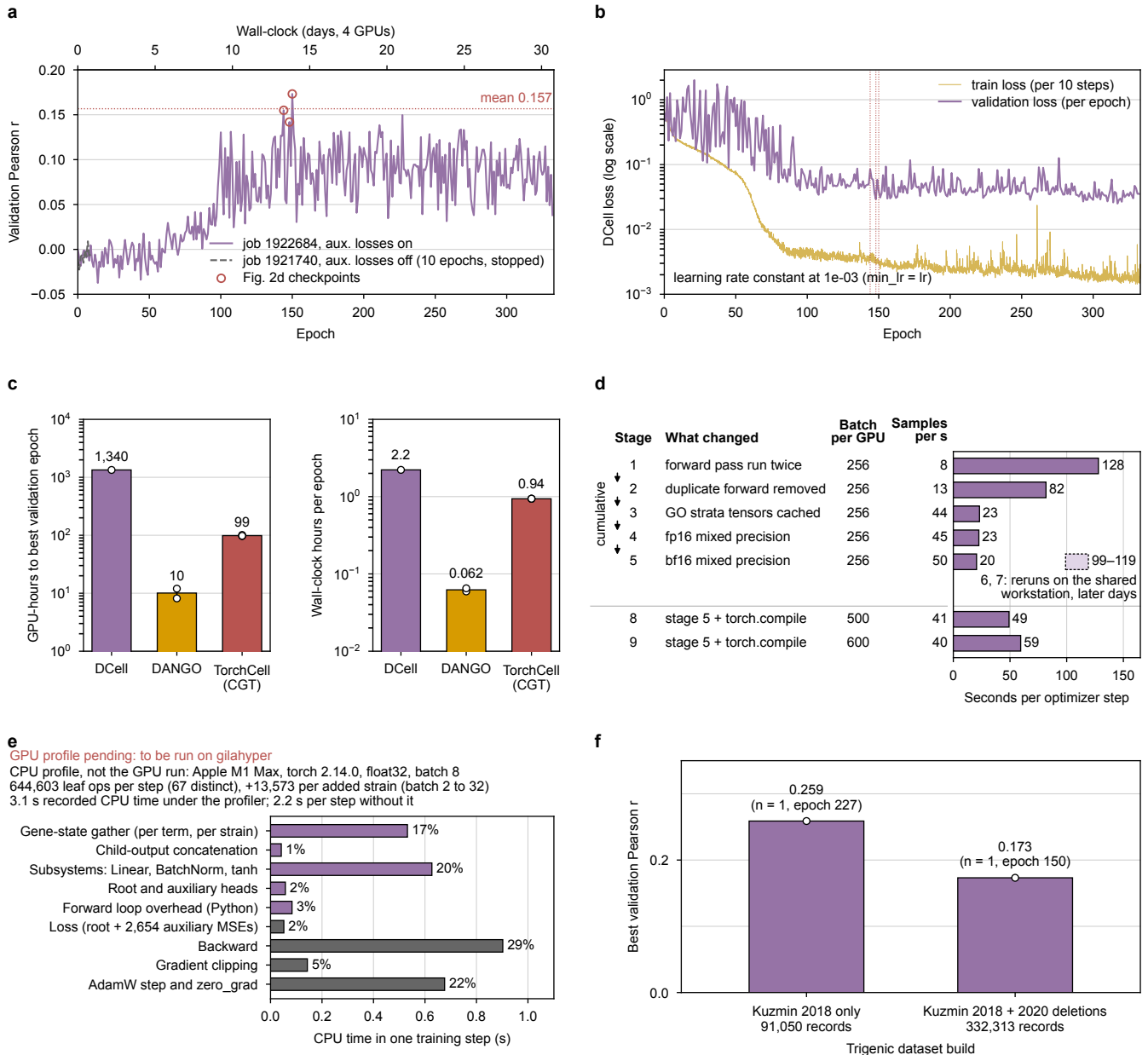
Supplementary Figure 11 DCell training on the trigenic interaction task: one run, its checkpoint statistic, and its cost.
