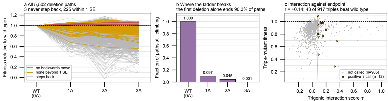
Figure 4: All 5,502 measured deletion paths through the pcl6 \Delta pcl7 \Delta screen, the step at which each route stops climbing, and trigenic interaction against endpoint fitness. Generated by experiments/010-kuzmin-tmi/scripts/pcl6_deletion_paths.py .
