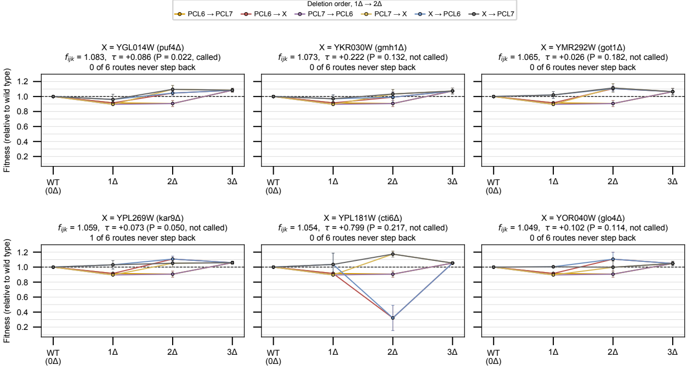
Figure 5: The six highest-fitness triples of the screen, all six deletion orders each, error bars 1 SE. Two of the six routes pass through the paralog double, whose fitness is one value for the whole screen. Generated by experiments/010-kuzmin-tmi/scripts/pcl6_deletion_paths.py .
