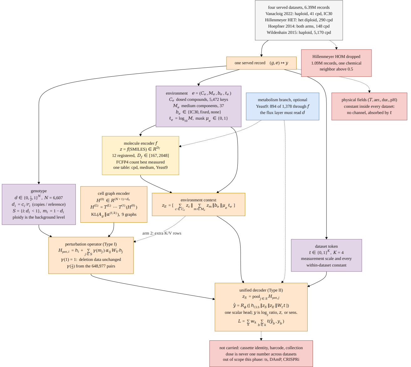
Figure 2: One input representation and one decoder for the four kept datasets, in the notation of the cell graph transformer: N genes, d_h the hidden width, S the perturbed set, H_{pert} the Type I output, R_\phi a Type II readout. Gray is a served dataset, purple a per-record input channel, yellow the fixed embedding table, orange a computation, blue the optional metabolism branch, red what the representation drops or does not carry. The genotype is a per-gene functional dose whose background level is the ploidy, and it scales the perturbation operator through \gamma(m_j) . The environment is a compound set and a medium set through the shared molecule encoder, a dose-basis token and a masked log molar value, pooled into one context z_E . The dataset token t carries the measurement scale and every physical field, because each of those is constant within a dataset. The decoder is one scalar head over the concatenation.
