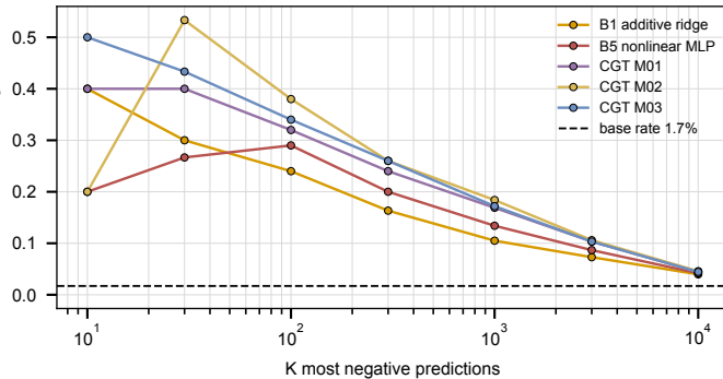
Random over records (the published split)
