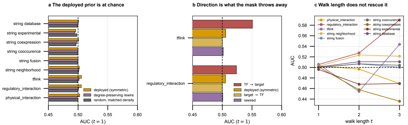
Figure 12: (a) All nine graphs in the orientation the model actually uses. (b) The two directed graphs, by orientation. (c) Longer walks do not recover anything; several graphs fall below chance by t = 3 .
