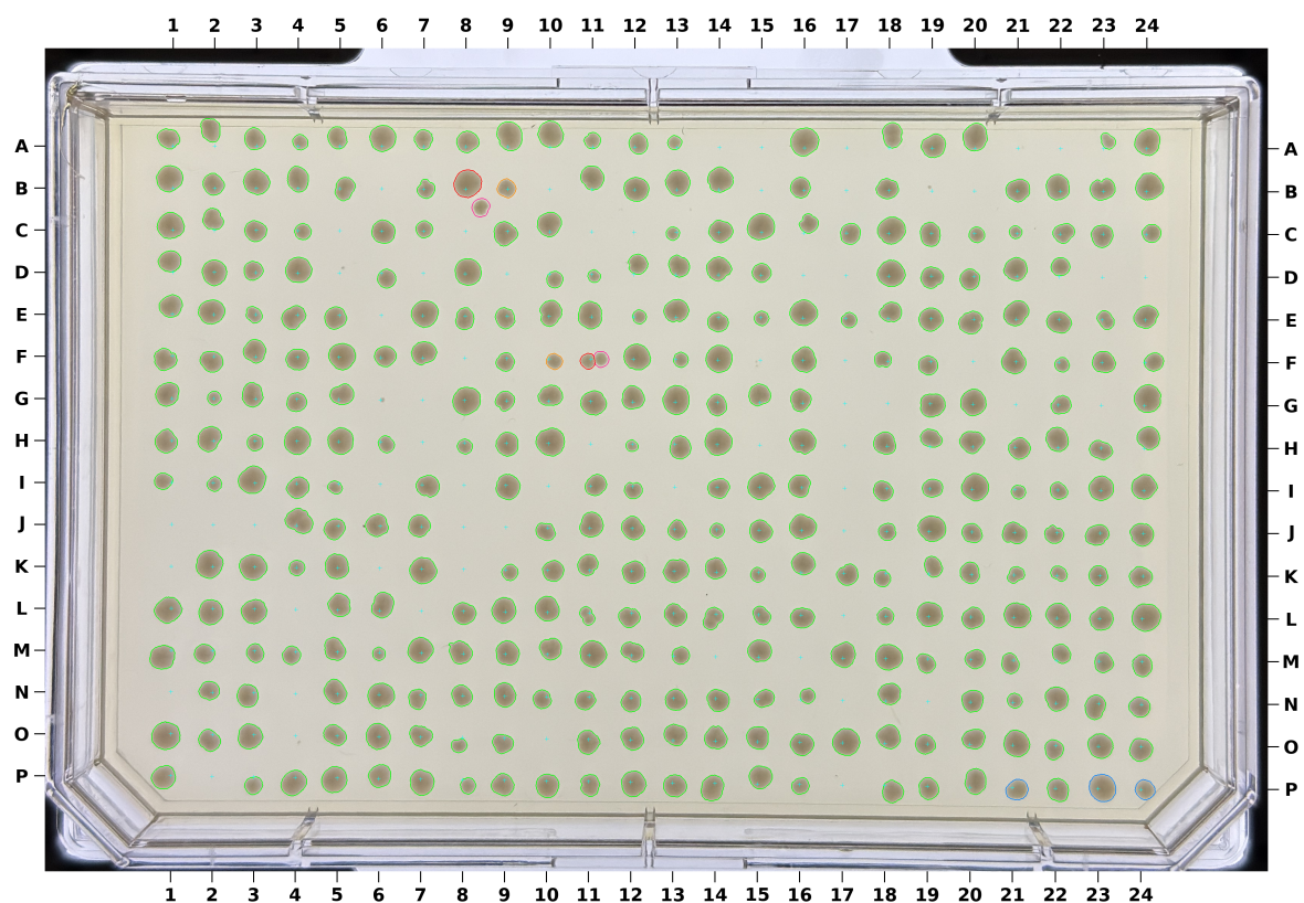
Fig. 10 Run 4, plate P1 (5 nL, OD 1.0, 48 h). 320 of 384 wells occupied, 6/6 blanks empty, WT CV 0.153.
