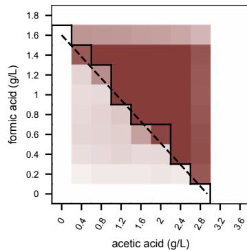
excess over Bliss, mean -0.45 [-0.54, -0.37]
