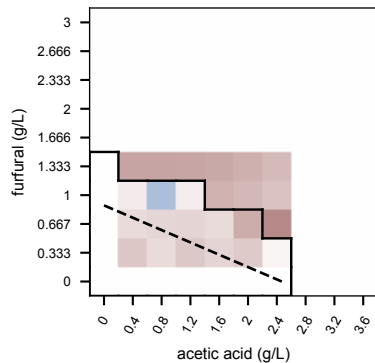
excess over Bliss, mean -0.08 [-0.14, -0.02]
