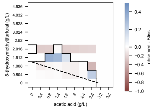
excess over Bliss, mean -0.02 [-0.04, 0.01]
