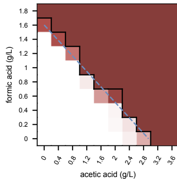
ex27: observed fitness
