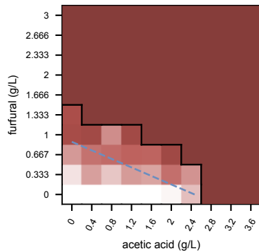
ex26: observed fitness
