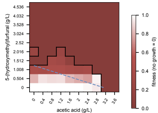
ex28 (flagged): observed fitness
