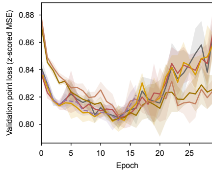
Held-out loss by epoch
