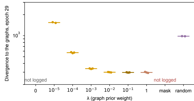
How close the attention gets
