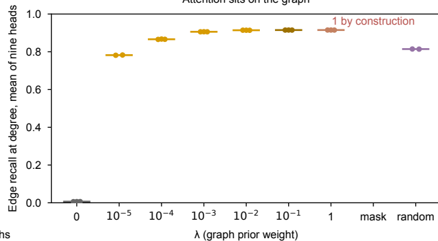
Attention sits on the graph
