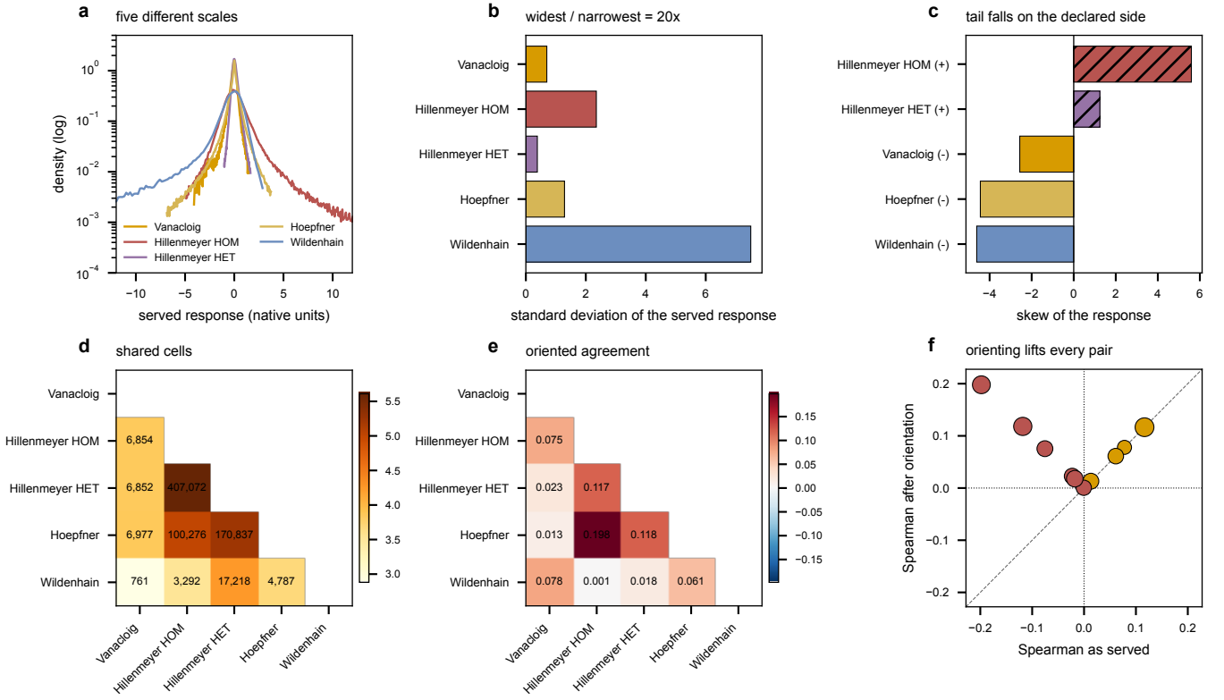
Figure 2: The five datasets disagree about the scale of the response and about which sign means a sick strain. a , Response density per dataset on a log scale, where the phenotype lives; the distributions differ in width by a factor of twenty and in which tail is heavy. b , Standard deviation of the served response, the factor a pooled squared-error loss would weight by. c , Skew beside the sign each source declares for a sick strain, an independent check on the declared convention; hatching marks the two datasets whose sources use the opposite sign. d , Shared (gene, compound) cells for every dataset pair on a log color scale, which is where agreement can be observed at all. e , Spearman correlation on those shared cells after orienting both datasets to one convention. f , The same pairs as served against oriented, point area by shared cells; red points are pairs whose sources disagree about the sign, and every pair moves above zero once oriented.
