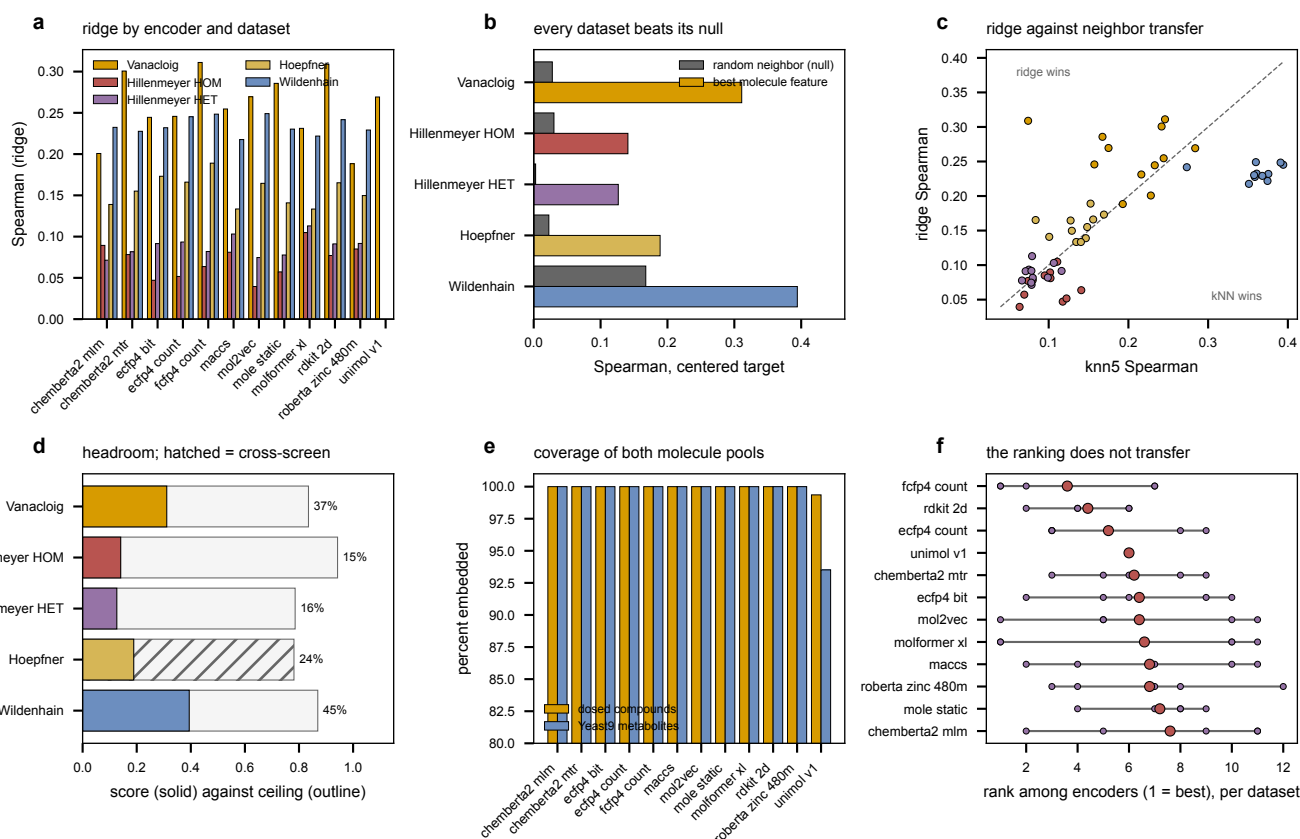
Figure 5: Molecule features carry signal in every dataset, and no single encoder choice is supported across them. Compound cold-start, centered target. a , Every encoder and dataset under ridge. b , The best molecule feature against the no-feature null per dataset; every dataset clears its null, and Wildenhain’s null is by far the highest because a random neighbor among 5,170 compounds is already informative. c , Ridge against nearest-neighbor transfer, one point per dataset and encoder; points below the diagonal are datasets where neighbor transfer wins, which is every Wildenhain point and most Hillenmeyer points. d , The best score against the ceiling. The Hoepfner bar is hatched because its ceiling comes from the cross-screen estimator of Table 9 rather than from a served uncertainty, so it is not the same quantity as the other four. e , What share of each molecule pool an encoder can embed, the 5,472 dosed compounds beside the 894 structure-bearing Yeast9 metabolites; only the three-dimensional encoder falls short, on the ions and metal salts it cannot build a conformer for, so coverage is not what separates these encoders. f , Each encoder’s rank among the twelve on each dataset, the line spanning its best and worst rank and the large mark its mean; the spans overlap almost completely.
