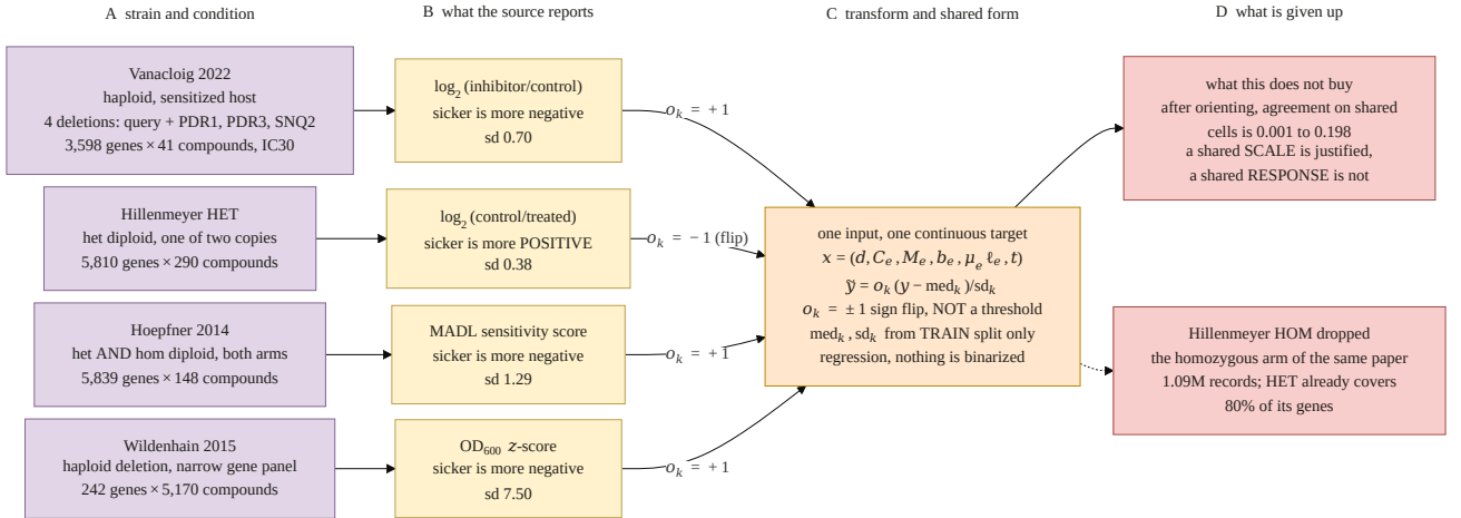
Figure 3: Four datasets, one input tuple and one continuous target, with two scalars per source doing all the work. One row per kept dataset, read left to right through four layers. a , What the record is: the strain, its ploidy and the size of the gene and compound panel. Vanacloig's four deletions are the queried gene plus the three efflux regulators that make its host drug-sensitive. b , What the source reports, in its own units and sign convention; the two \log_2 ratios point in opposite directions because one is taken treated over control and the other control over treated, and MADL is the median absolute deviation logarithmic score. c , The transform and the shared form it produces. The orientation factor o_k multiplies by plus or minus one, so three datasets pass through unchanged and only Hillenmeyer HET flips; it is a sign flip on a continuous number and never a threshold, and the median and standard deviation come from the training split alone. d , What is given up: the homozygous arm of Hillenmeyer 2008, dropped because its heterozygous sibling already covers 80 percent of its genes, and the measured limit that orienting buys a shared scale rather than a shared response. Per-dataset counts are in Table 7.
