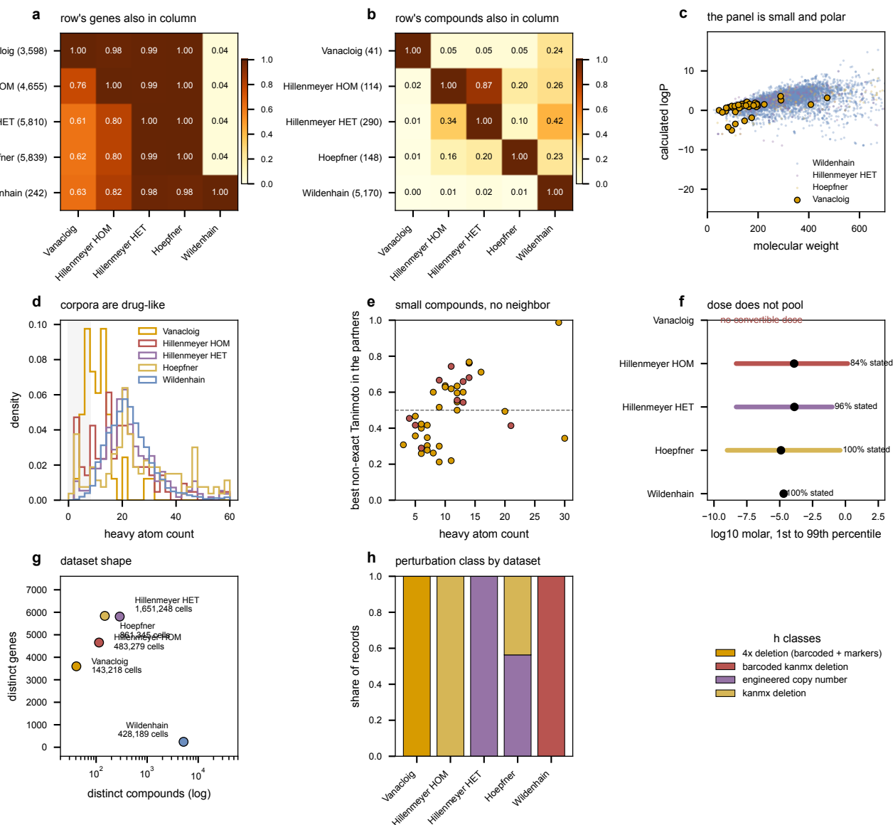
Figure 4: Genes overlap heavily, compounds barely, and the application panel sits outside the chemistry the partners cover. a , Share of the row dataset’s genes that the column dataset also measures, with each dataset’s gene count. b , The same for compounds, where the shares collapse. c , Molecular weight against calculated logP for every dosed compound, the Vanacloig panel outlined; the partner libraries are drug-like and the application panel is small and polar. d , Heavy atom count; the shaded band below 8 heavy atoms is where a substructure fingerprint carries almost no bits, which is where most of the hydrolysate panel sits. e , Each Vanacloig compound’s best non-exact Tanimoto in the partner union against its size, showing that the compounds without a neighbor are the small ones. f , The molar range each dataset spans, 1st to 99th percentile, with the share of records stating a convertible dose. g , Distinct compounds against distinct genes, with each dataset’s measured cell count in its label. h , Perturbation class by dataset.
