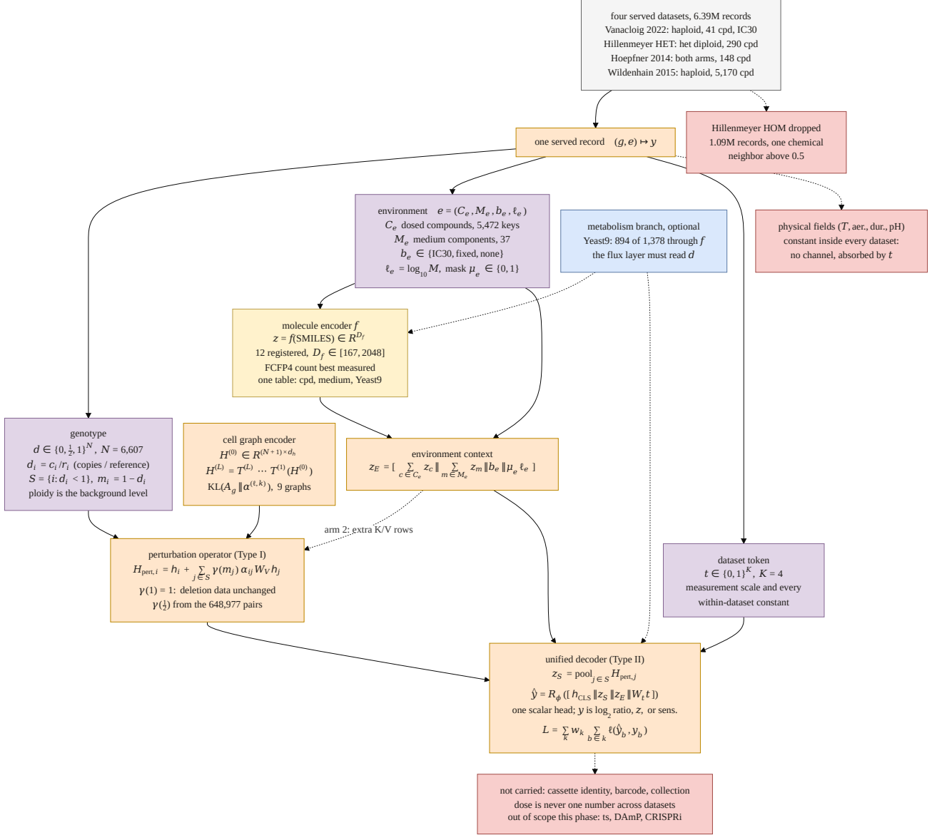
Figure 6: One input representation and one decoder for the four kept datasets. Drawn in the notation of the cell graph transformer: N genes, d_h the hidden width, S the perturbed set, H_{\text{pert}} the Type I output, R_\phi a Type II readout. Gray is a served dataset, purple a per-record input channel, yellow the fixed embedding table, orange a computation, blue the optional metabolism branch, red what the representation drops or does not carry. The genotype is a per-gene functional dose whose background level is the ploidy, and it scales the perturbation operator through \gamma(m_j) . The environment is a compound set and a medium set through the shared molecule encoder, a dose-basis token and a masked log molar value, pooled into one context z_E . The dataset token t carries the measurement scale and every physical field, because each of those is constant within a dataset. The decoder is one scalar head over the concatenation.
