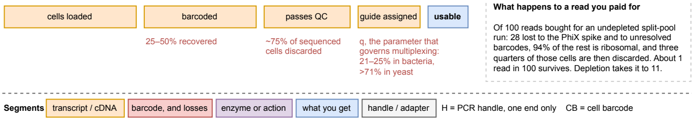
Figure 6: The whole experiment, and where each stage costs you cells, molecules or identity. Two symbols recur in panel (b) and are worth having before reading it: H is the PCR handle, attached at one end only during barcoding, and CB is the cell barcode. The full color key is repeated at the foot of the figure. (a) The stages. Everything outside the shaded block is common to both method families; only the way cell identity gets written differs, which is the argument sections 3.1 to 3.3 make in detail. Fragmentation is drawn as its own stage because its position relative to rRNA depletion is what section 3.5 corrects, and because it determines what a count means; the $99,000 that depletion is worth at genome scale is derived in section 3.5, and the 25 to 50% recovery drawn in panel (c) is section 3.1's. (b) The same physical cutting, with opposite consequences. In bulk RNA-seq every piece of a molecule can be sequenced, so a long transcript yields proportionally more reads and the length has to be divided back out, which is what FPKM and TPM are for. In a 3'-counting single-cell assay only the barcode-proximal piece keeps the outer handle, so exactly one fragment survives per amplified copy whatever the length, and UMI collapse reduces the copies to one count. Length drops out by construction; see section 2.4. (c) The funnel. A budget is made of these fractions rather than of the chemistry: cells are lost at recovery, at QC and at guide assignment, and reads are lost separately to spike-in, to ribosomal sequence and to cells that are later discarded. Composed from the protocols as described in sections 3.1, 3.2 and 3.5, not traced from any published figure. Drawn at true Nature print size in notes/assets/drawio/perturb-seq-workflow.drawio. Every number drawn by hand in this figure is sourced in table 27.
