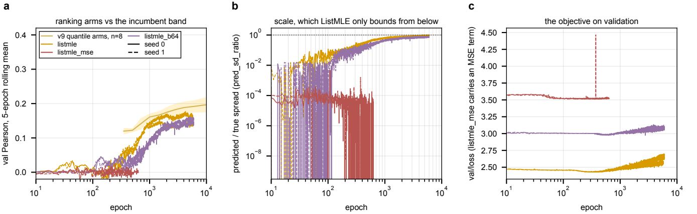
Figure 6: The anchored ranking runs collapse to the mean predictor by epoch 250 and the pure ranking runs stay under the long-budget band. a , validation Pearson of all six runs against the long-budget arm band. b , predicted over true spread; the anchored runs fall off the bottom by epoch 250 while the pure runs climb from 0.05 toward 1. c , the objective on validation, which bottoms at epochs 290 to 630 and rises after, as every other objective in fig. 2 does. Generated by pearson_round_readout.py--roundlistmle .
