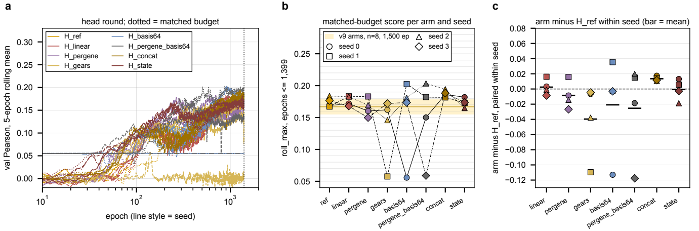
Figure 7: Only H_{\text{concat}} is above H_{\text{ref}} in every seed, by +0.0135 over four seeds, a small resolved effect; three runs never left the plateau. a , validation Pearson (5-epoch rolling mean) of all 32 runs, color by arm, line style by seed; the dotted line is the matched budget. b , \text{roll\_max} at epochs \leq 1,399 per arm and seed, lines joining one seed's arms; the band is the eight v9 long-budget arms at 1,500 epochs. c , the paired difference against H_{\text{ref}} within seed, bar at the mean. Generated by head_round_readout.py .
