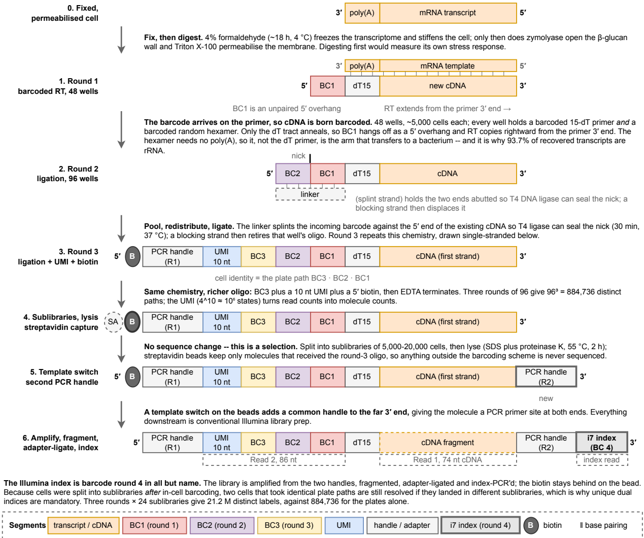
Figure 2: Cell identity in split-pool barcoding is assembled onto the transcript itself, which is what removes the need to ever physically isolate a cell. Seven strand states in the yeast-optimised SPLiT-seq workflow of section 3.1 [2], each arrow annotated with the chemistry that produces the next. Strands are drawn 5' left to 3' right, so the barcode block grows leftward with each round while the cDNA body stays fixed — the visual point being that a cell's address is written in three instalments, and a cell is identified by the path it took through three 96-well plates rather than by ever having been alone in a well. That is the whole economic argument for the method: 96^3 distinct paths cost three plates, not 10^6 containers. Two states are drawn double-stranded because that is where the mechanism is easy to get wrong. At round 1 the mRNA template lies antiparallel above the tracked strand, showing BC1 as an unpaired 5' overhang, and showing that the random hexamer rather than the poly-dT primer is the arm that carries the method to transcripts without a poly(A) tail — the single change that lets the same chemistry work in bacteria [5, 6]. At round 2 the linker strand base-pairs underneath and a tick marks the nick T4 ligase seals; ligation is templated by that splint, which is why an unretired barcode from a previous well would scramble the address and why a blocking strand follows every round. The 5' biotin added in round 3 is not a label but a selection handle: streptavidin capture at the next step discards every molecule that fell out of the scheme, so incompletely barcoded material is removed before it can consume sequencing. Composed from the protocol as described in section 3.1, not traced from any published figure; every parameter shown is sourced there. Drawn at true Nature print size in notes/assets/drawio/splitseq-barcoding.drawio.
