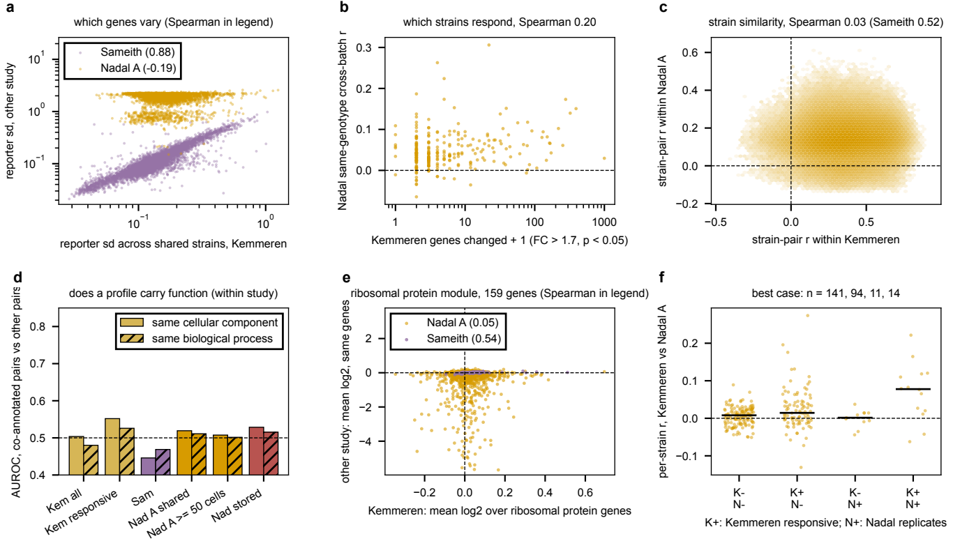
Figure 13: Agreement at levels a per-gene correlation misses, on the 1,002 shared deletions. a , a reporter's sd across the shared strains, Kemmeren against Sameith and against Nadal-Ribelles A. b , Kemmeren's changed-gene count per deletion against the genotype's cross-batch replication in Nadal-Ribelles A. c , strain-pair correlation within Kemmeren against the same pair within Nadal-Ribelles A. d , within one study, the AUROC of the pair correlation for pairs annotated to one GO cellular-component or biological-process term of 5 to 100 genes against other pairs. e , mean log 2 over 159 cytosolic ribosomal protein genes per strain, Kemmeren against Nadal-Ribelles A and against Sameith. f , per-strain cross-study r by whether Kemmeren calls the deletion responsive (K+) and whether its Nadal-Ribelles profile replicates across batches at r \geq 0.1 (N+); bars are medians. Generated by cross_study_structure.py .
