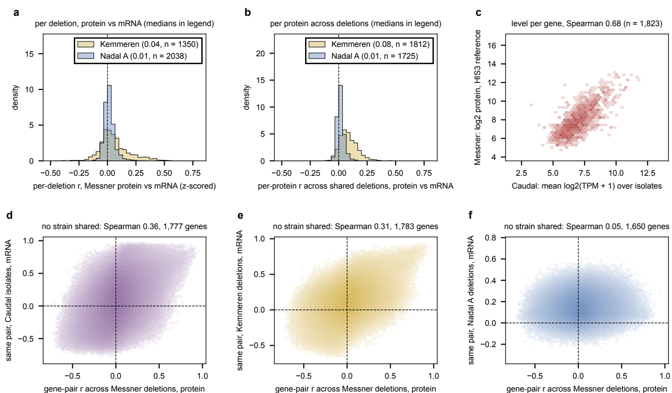
Figure 14: The Messner 2023 knockout proteome against three expression panels. a , per shared deletion, the Pearson between its protein and mRNA log 2 ratios (z-scored per gene across strains) for Kemmeren and for Nadal-Ribelles A. b , per protein, the Pearson across shared deletions. c , abundance level per gene, protein in the HIS3 reference against mean expression over the Caudal isolates. d–f , gene-pair co-variation: the correlation of two genes across Messner’s deletions (protein) against the same pair across Caudal’s isolates, Kemmeren’s deletions and Nadal-Ribelles A’s deletions (mRNA), log-count density. Generated by proteome_expression_covariation.py .
