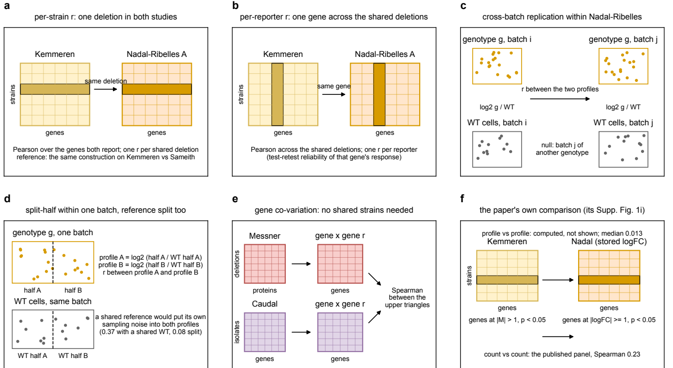
Figure 8: The comparison designs. a , per-strain: one deletion’s profile in each study, correlated over the genes both report. b , per-reporter: one gene’s response across the shared deletions in each study. c , cross-batch replication inside Nadal-Ribelles: one genotype’s cells in two cartridge batches, each pseudobulked against the wild-type cells of its own batch; the null pairs batch j of another genotype. d , split-half inside one batch with the wild-type cells split too, so the two profiles share no cell. e , gene co-variation: within one panel the correlation of every gene pair across that panel’s strains, then the two panels’ upper triangles compared, which needs no shared strain and admits the Caudal isolates. f , the paper’s own comparison: DE-gene counts per genotype (published) and the profile correlation its script computes (not published). Generated by comparison_designs.py .
