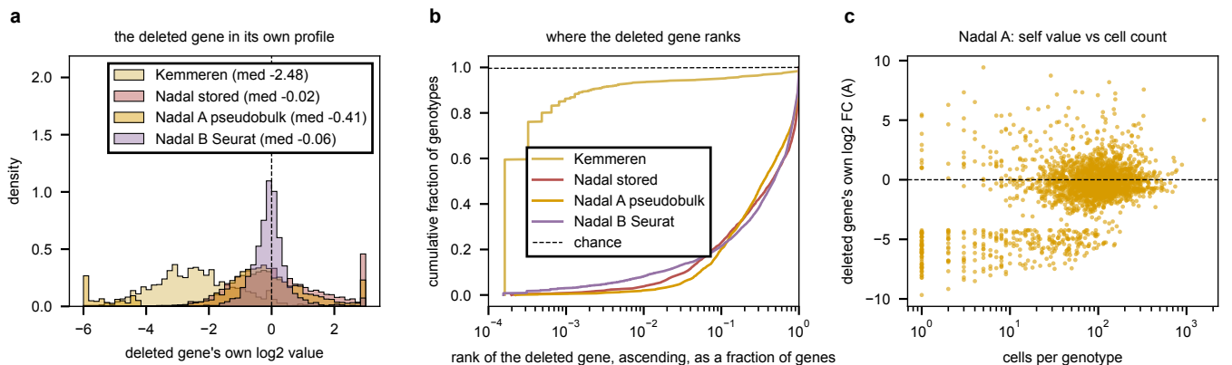
Figure 11: The deleted gene in its own profile. a , the deleted gene's own log 2 value per genotype for Kemmeren and three Nadal-Ribelles statistics. b , cumulative distribution of the deleted gene's ascending rank as a fraction of genes in the profile, log axis; the dashed diagonal is chance. c , for the pseudobulk statistic, the deleted gene's own value against the cells behind the genotype; the band near -5 to -8 at low counts is the pseudocount floor of a near-empty pseudobulk. Generated by nadal_identify_deletion.py .
