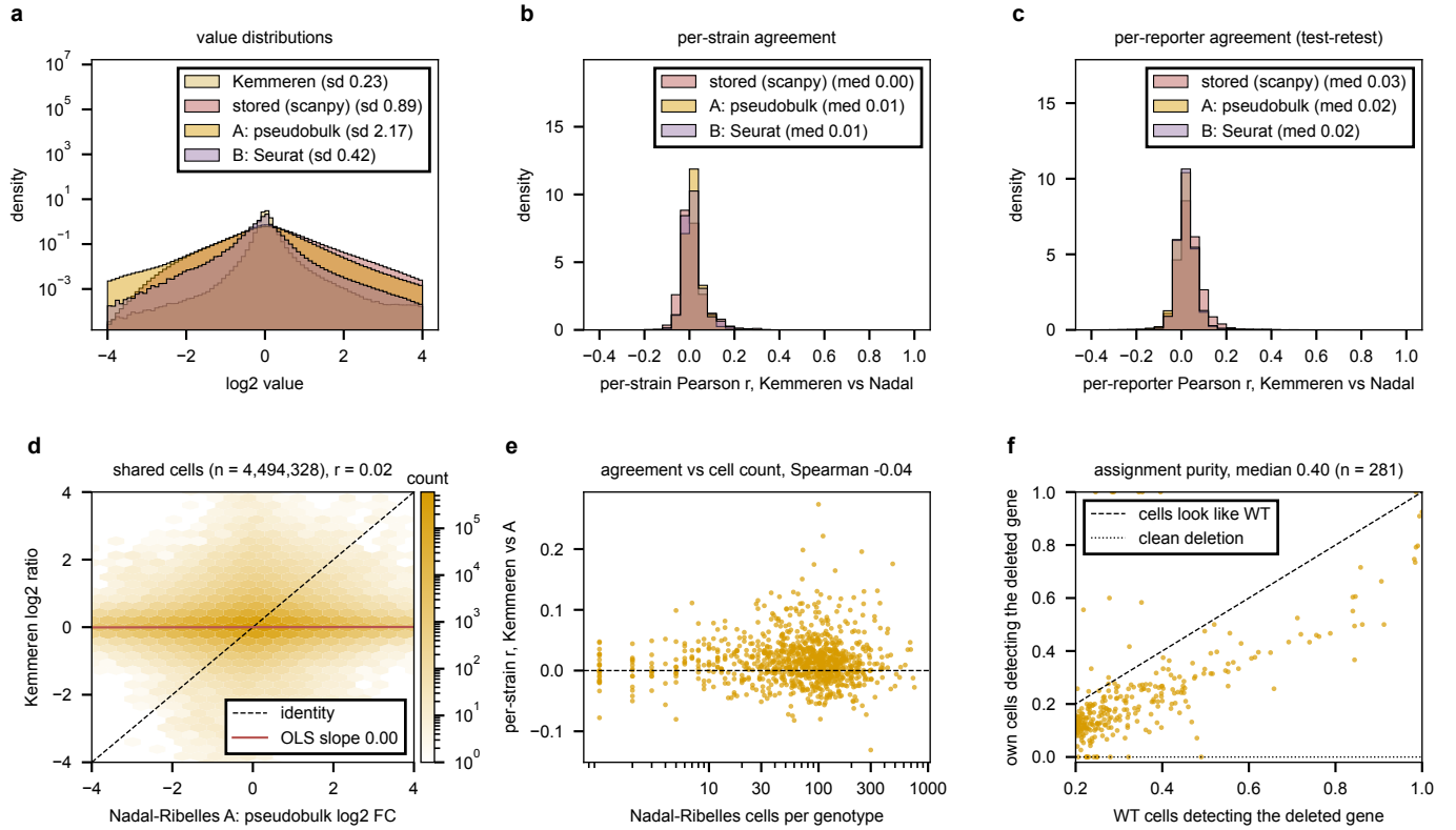
Figure 10: Recomputing the Nadal-Ribelles fold change from the single-cell object, and why it does not help. a , log 2 values of Kemmeren and of three Nadal-Ribelles versions: as stored, the bulk-like pseudobulk ratio (A) and Seurat's avg_log2FC (B). b , per shared deletion, the Pearson across reporters with Kemmeren for each version; c , the same per reporter across shared strains. d , Kemmeren against A on every shared cell. e , per-strain agreement of A against the cells behind the genotype. f , assignment purity: for each genotype whose deleted gene wild type detects in at least a fifth of cells, the fraction of the genotype's own cells detecting that gene against the wild-type fraction; the dashed identity is what cells that are not the genotype look like, the dotted zero a clean deletion. Generated by cross_study_recomputed.py from nadal_pseudobulk_recompute.R and nadal_assignment_purity.R .
