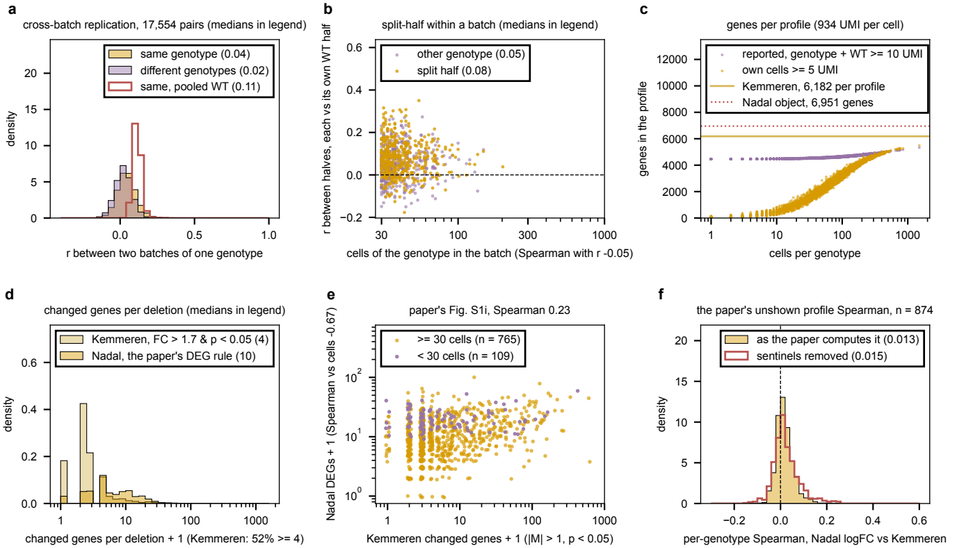
Figure 12: Within-study replication, coverage, and the paper's own deleteome comparison. a , Pearson between two batches of one genotype (pseudobulk against the batch's own wild-type cells), the different-genotype null with matched cell counts, and the same-genotype value with a pooled wild-type reference. b , split-half within one batch, each half against its own half of the wild-type cells, against cells per genotype; gray, the other-genotype null. c , genes per profile: covered by the genotype's own cells at five or more UMI, and reported under the summed-UMI rule; lines at Kemmeren's reporters per profile and at the genes in the single-cell object. d , changed genes per deletion under each study's own rule. e , the paper's Supplementary Fig. 1i reproduced from its released objects, shaded by cells per genotype. f , the per-genotype profile Spearman the paper's script computes and does not show, with and without the sentinel genes. Generated by nadal_replication_coverage.py from nadal_batch_replication.R and nadal_paper_deleteome_comparison.R .
