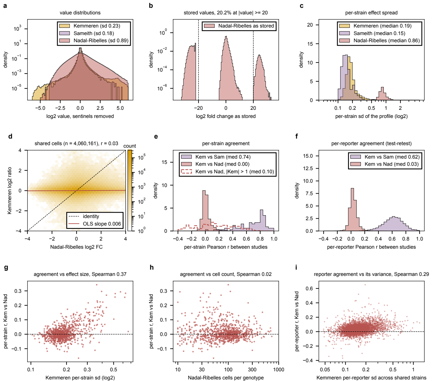
Figure 9: Three single-deletion expression panels compared, base medium only. a , log 2 values of each panel with the Nadal-Ribelles sentinels removed; the two platforms sit on different scales. b , Nadal-Ribelles values as stored, with the \pm 20 lines: 20.2% of cells are the zero-mean sentinel. c , per deletion, the standard deviation of its profile across reporters. d , Kemmeren against Nadal-Ribelles on every shared (strain, gene) cell, log-count density, with the identity and the fitted slope. e , per shared deletion, the Pearson across reporters between its two profiles: Kemmeren vs Sameith ( n = 82 ), Kemmeren vs Nadal-Ribelles ( n = 914 ), and the latter over only the reporters with |\log_2| > 1 in Kemmeren (dashed, n = 368 strains). f , per reporter, the Pearson across shared strains between its two response vectors, the test-retest reliability behind the ceiling. g , the per-strain agreement of e against the strain's Kemmeren spread; h , against the number of cells behind its pseudobulk; i , the per-reporter agreement of f against the reporter's Kemmeren spread across the shared strains. Generated by cross_study_ko_expression.py .
