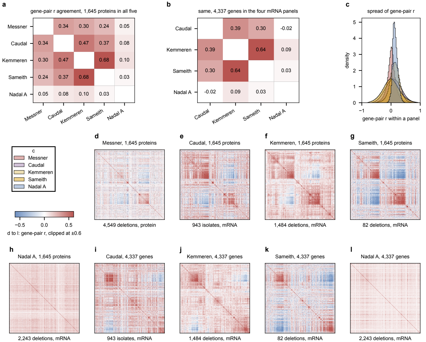
Figure 15: Gene-pair co-variation in every panel. Within a panel, two genes get one Pearson across that panel's own strains; no strain is aligned between panels. a , Spearman between the upper triangles of two panels' gene-by-gene matrices on the 1,645 proteins measured in all five panels. b , the same on the 4,337 genes measured in the four mRNA panels. c , the distribution of the gene-pair r within each panel on the protein gene list. d–h , the five matrices on the protein gene list, and i–l the four mRNA matrices on the expression gene list, every matrix in the ordering given by average-linkage clustering of Kemmeren's matrix on that gene list, so a block in Kemmeren can be looked for at the same place in every other panel; color clipped at \pm 0.6 , with the key for c and for the matrices in the first cell of the block. Sameith has 82 single deletions, Nadal-Ribelles A the 2,243 deletions with at least 50 cells. Generated by gene_covariation_all.py .
