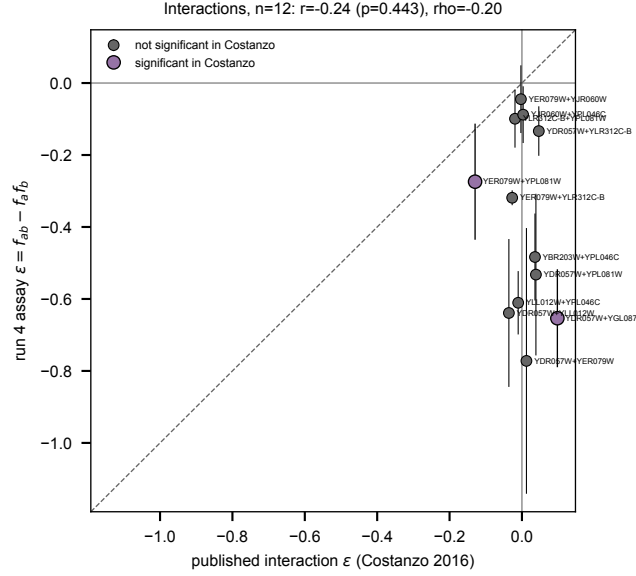
Fig. 9 Run 4 \varepsilon against published Costanzo \varepsilon , the two Costanzo-significant pairs marked. Every point sits below zero and the published spread is not recovered. This panel is published as the record of a diagnosed artifact, not as a measurement of epistasis.
