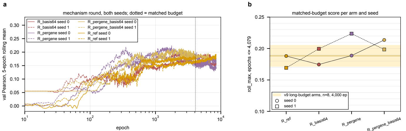
Figure 4: The mechanism round. a , validation Pearson of all eight runs (solid seed 0, dashed seed 1); the dotted line is the matched budget. b , the matched-budget score per arm and seed against the long-budget arm band at 4,000 epochs. Generated by mech_round_readout.py .
