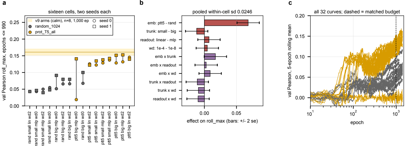
Figure 3: The v10 grid at a matched budget. a , every cell’s two seeds at epochs \leq 990 , sorted by cell mean and colored by embedding, against the eight long-budget v9 arms at 1,000 epochs ( 0.161 \pm 0.010 , calm embeddings, band is one standard deviation across arms). b , main effects and two-way interactions with \pm 2 standard errors from the pooled within-cell spread. c , all 32 validation curves; the dashed line is the matched budget. Generated by v10_grid_factorial.py .
